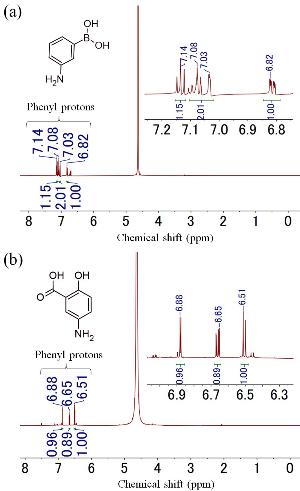
Fig. S1 ^1\text{H} NMR spectra of (a) 3APBA, and (b) Asal.
