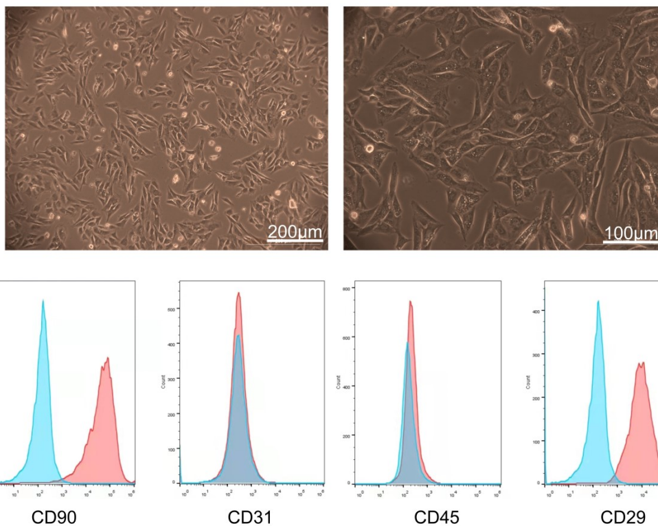
S.1 Morphological observation of ADSCs and characterization of flow cytometry (positive expression of CD90 and CD29; negative expression of CD31 and CD45).
