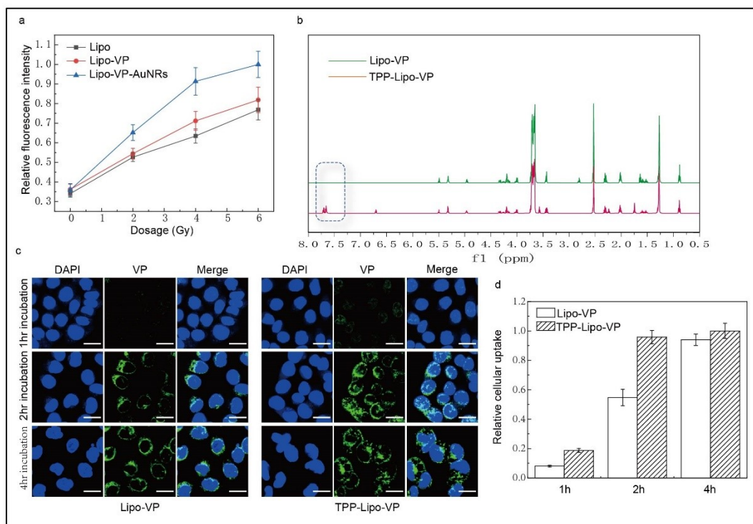
Supplementary Figure 1 (a) Relative SOSG fluorescence intensities from liposome samples at different X-ray doses. (b) 1 H NMR spectra of Lipo-VP and TPP-Lipo-VP. (c) Representative confocal laser scanning microscopy images of HCT 116 cells incubated with liposome samples for 1 h, 2 h and 4 h, respectively. Scale bar is 20 \mu m. Quantitative analysis of VP fluorescence intensity ( n=4 )
