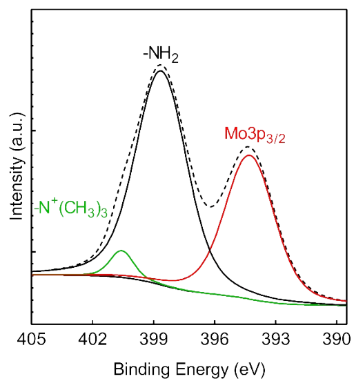
Fig. S2. Deconvoluted N1s spectra of SS-PDA-MCP.
