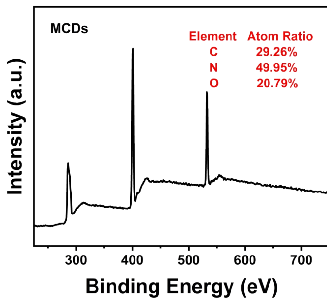
Figure S1. The XPS full-scan spectrum of MCDs.
