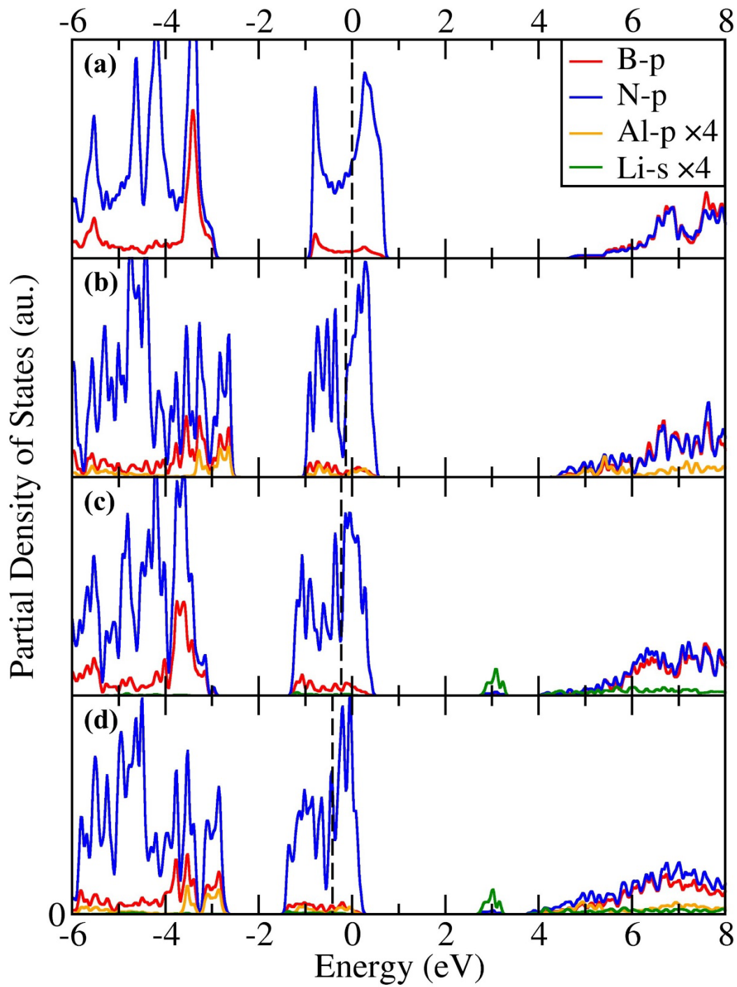
Figure S1 Partial density of states (PDOS) of (a) penta -BN 2 , (b) Li absorbed on penta -BN 2 , (c) Al-doped penta -BN 2 and (d) Li absorbed on Al-doped penta -BN 2
