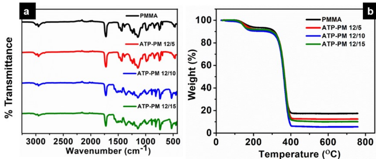
Figure S1. a) FT-IR spectra and b) TGA plot of PMMA, ATP-PM 12/5, ATP-PM 12/10, ATP-PM 12/15.
