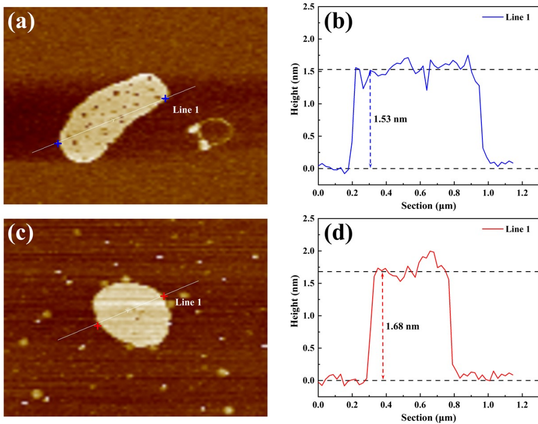
Fig. S2. AFM result of \text{Ta}_4\text{C}_3 nanosheets and the corresponding heights of lines.
