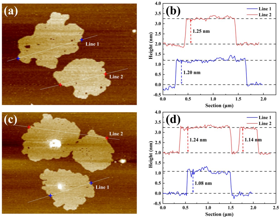
Fig. S1. AFM result of \text{Ta}_4\text{AlC}_3 nanosheets and the corresponding heights of lines.
