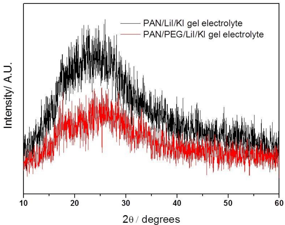
Figure S1: XRD pattern of (a) PAN/LiI/KI and (b) PAN-PEG/LiI/KI blend PGEs.
