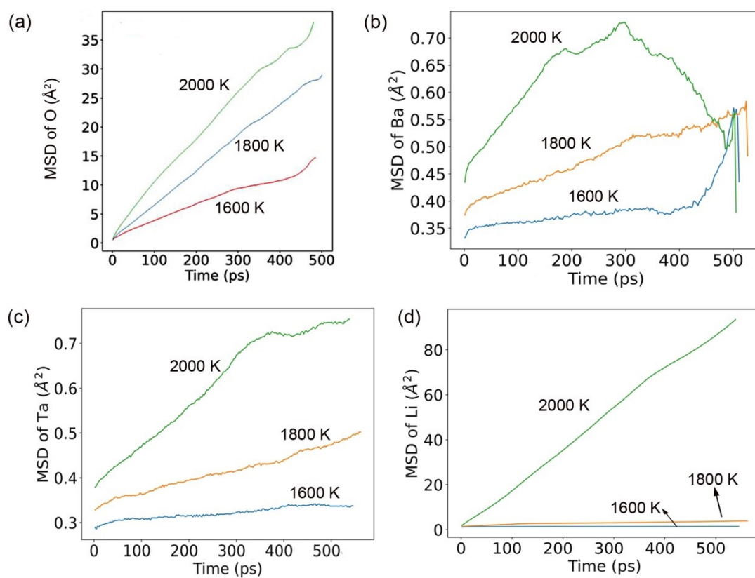
Figure S1. Mean square displacement (MSD) plot of (a) \text{O}^{2-} , (b) \text{Ba}^{2+} , (c) \text{Ta}^{5+} , and (d) \text{Li}^+ ions during AIMD simulations of three selected temperatures.
