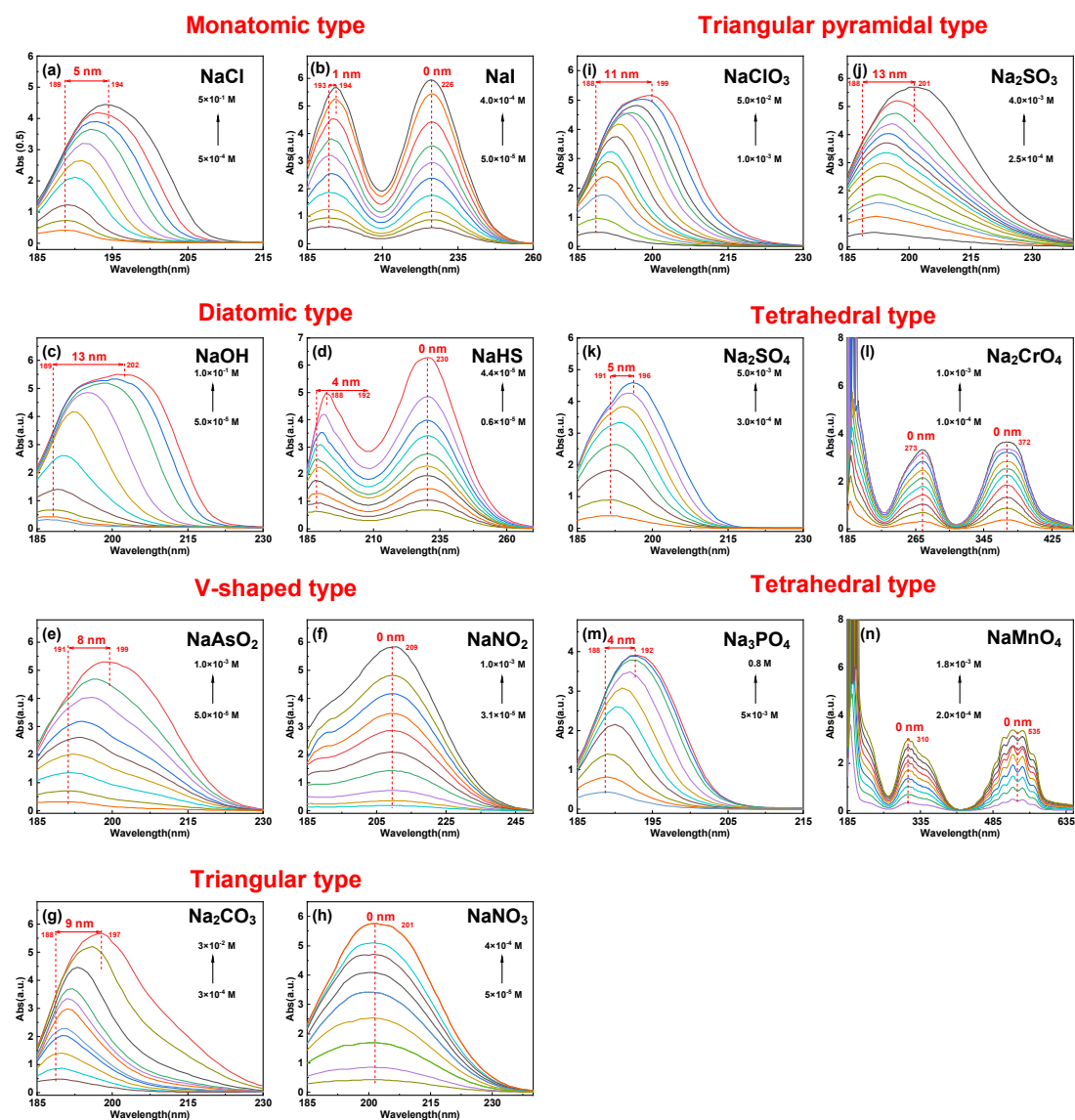
Fig. A.1. The absorption spectra of various anions with concentrations increase.
