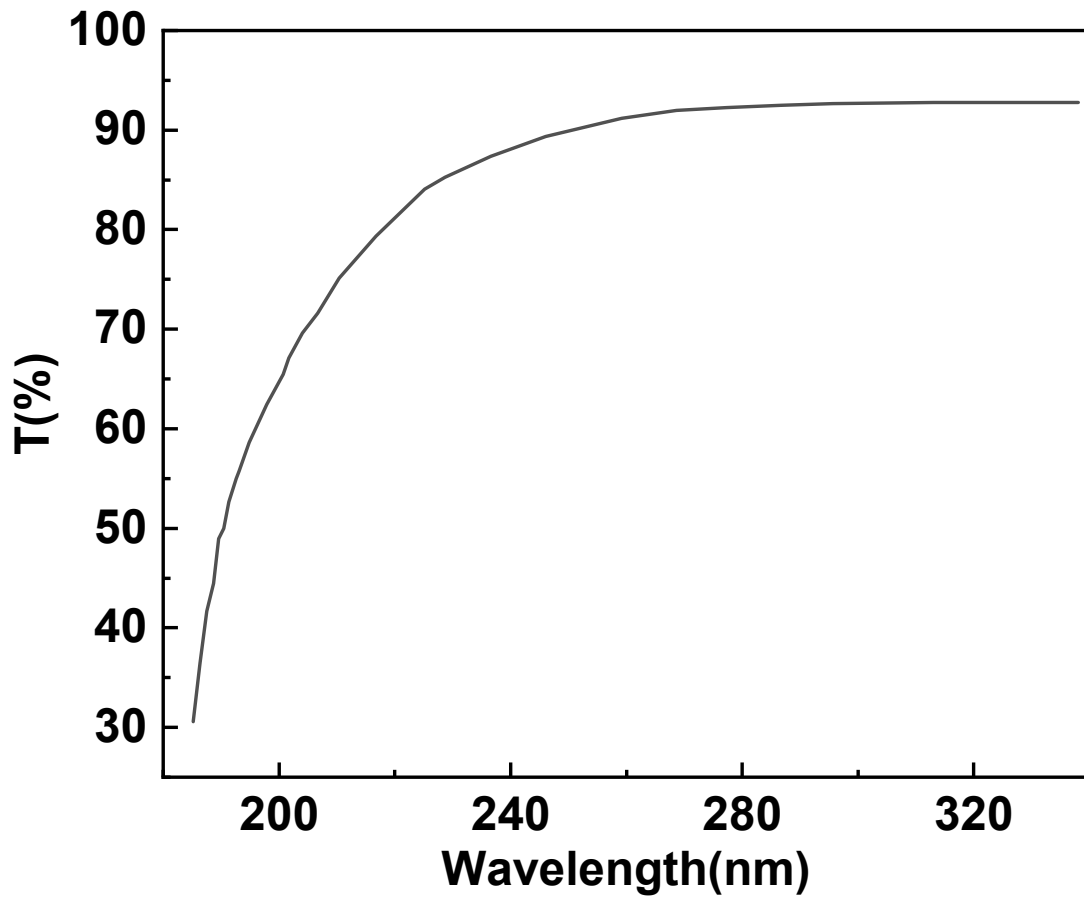
Fig. A.2. Transmittance of UV glass to different wavelengths of light.
