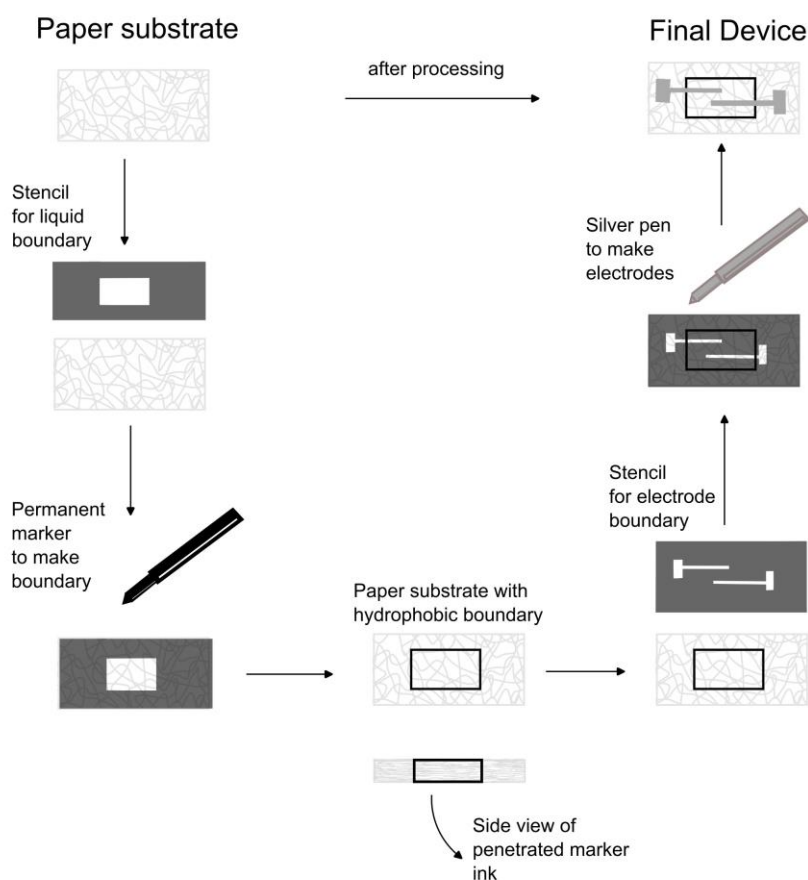
Scheme. 1 Design and fabrication of a paper chip for the droplet analysis.
