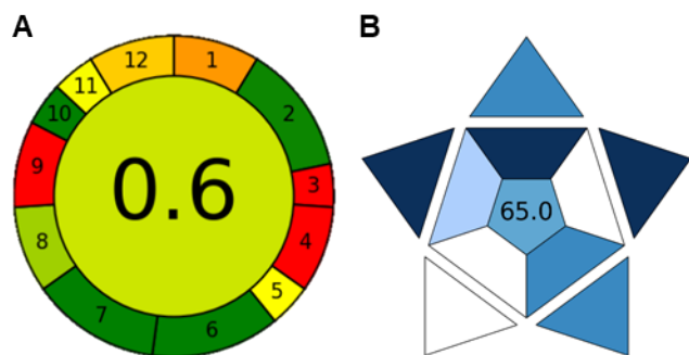
S-Figure 1: Results from the assessment of the greenness and applicability of the analytical method according “Analytical GREENness calculator (AGREE)” (A) and “blue applicability grade index (BAGI)” (B), ref. (1, 2).
