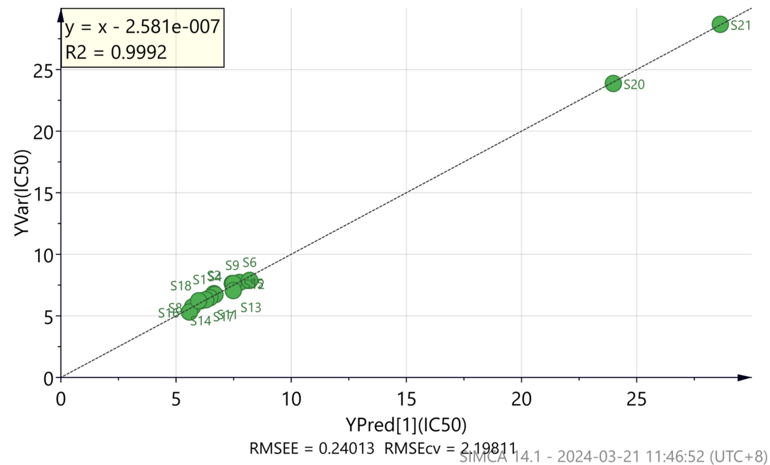
Fig. S3. The validation set of peak areas and IC 50 value correlations for FT-IR (A), UV (B) and HPLC (C). The training set of peak areas and IC 50 value correlations for FT-IR (D), UV (E) and HPLC (F).
