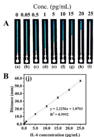
Fig. 5 (A) Photographs of devices with the IL-6 assay performed at various concentrations.
