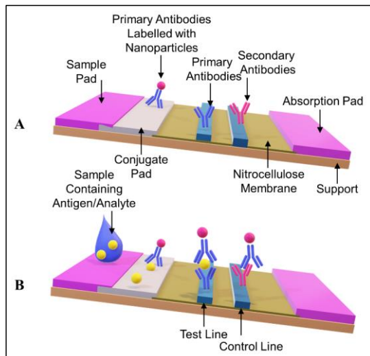
Fig. 3 (A) The architecture of a standard LFA. (B) Basic working principle of antibody-antigen-antibody sandwich LFA.
