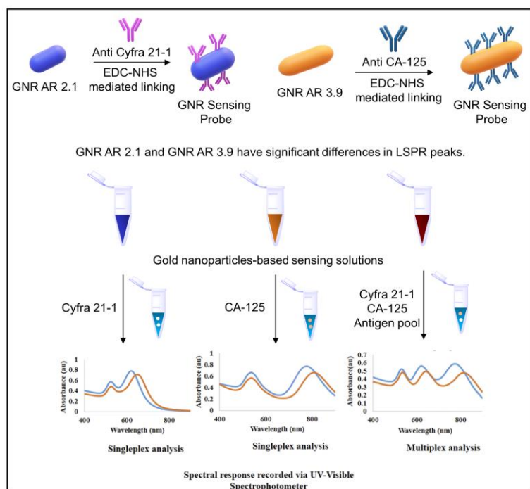
Fig. 13 The schematic depicting GNR probe development and the UV-visible spectroscopy-based spectral analysis of Cyfra 21-1 and CA-125 antigens. Reproduced/re-drawn with permission from ref 153499 . Copyright 2022 The Royal Society of Chemistry.
