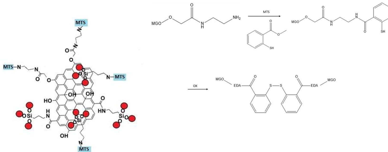
Figure SM1. Structure of functionalized M@GO.
