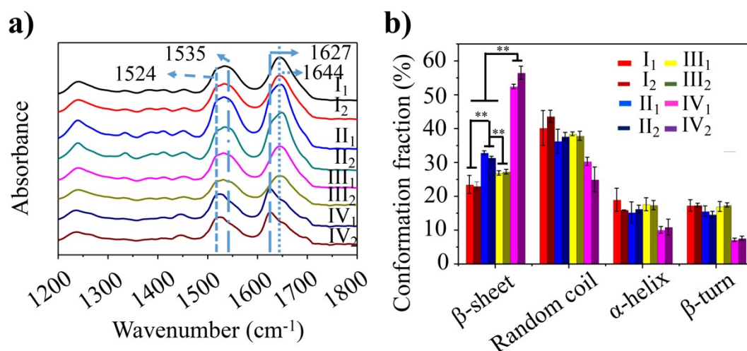
Fig. 1. FTIR spectra of silk films on pH test strips, with and without immobilized AChE. (1) The spectra without AChE; (2) The spectra with AChE. I: untreated, II: ultrasonic-treated, III: glycerol blend, IV: methanol-treated.
