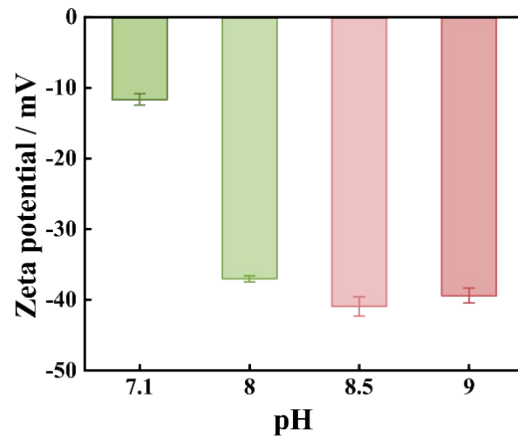
Fig. S3. Zeta potential of Met-EGCG NPs synthesized at different pH.
