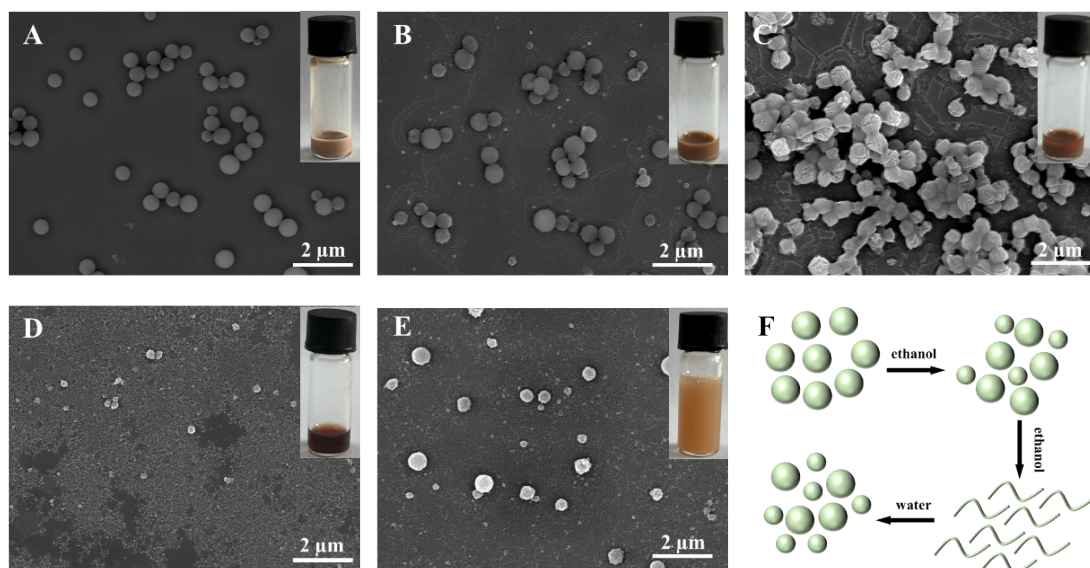
Fig. S1. SEM images and digital photograph (insert) of A. Met-EGCG NPs, B. 23% ethanol + Met-EGCG NPs, C. 28.6% ethanol + Met-EGCG NPs, D. 37.5% ethanol + Met-EGCG NPs, E. 37.5% ethanol + Met-EGCG NPs + 1 mL H 2 O, F. The formation mechanism for the controllable size of Met-EGCG NPs.
