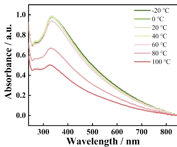
Fig. S8. UV-vis curves of Met-EGCG NPs after treated with different temperature.
