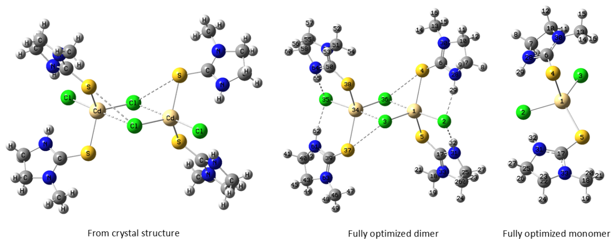
Figure S1. Figures of the dimers obtained from crystal structure and from fully optimized dimer and monomer.
