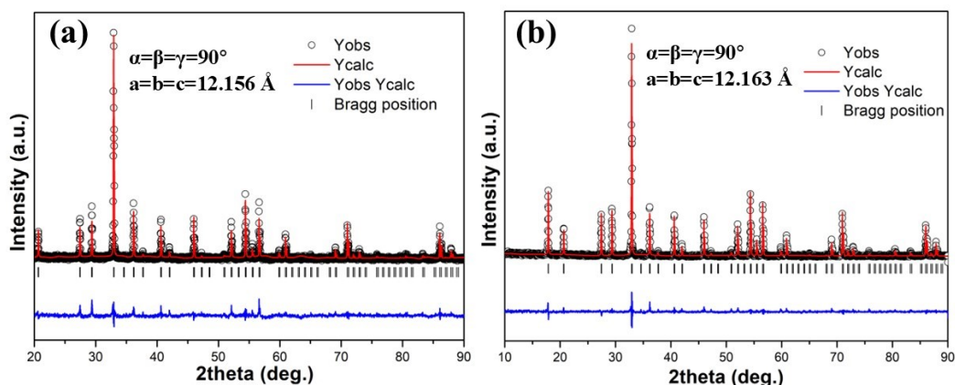
Figure S1. Refined XRD patterns of crystals: (a) Tm: TAGG, (b) TAGG.
