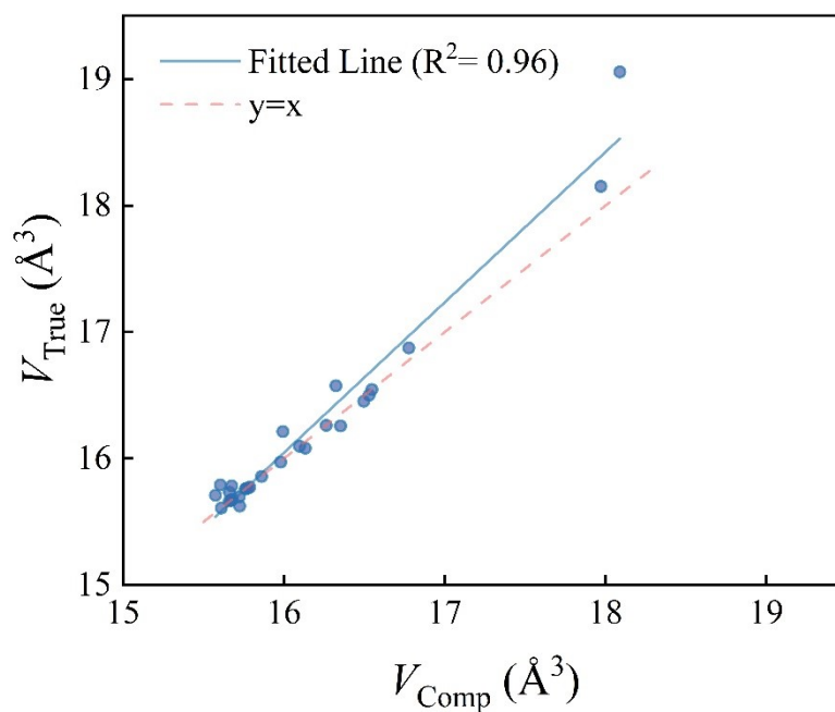
Fig. S2 Comparison between the true atom Voronoi volume and compute values based on Eq. 8.
