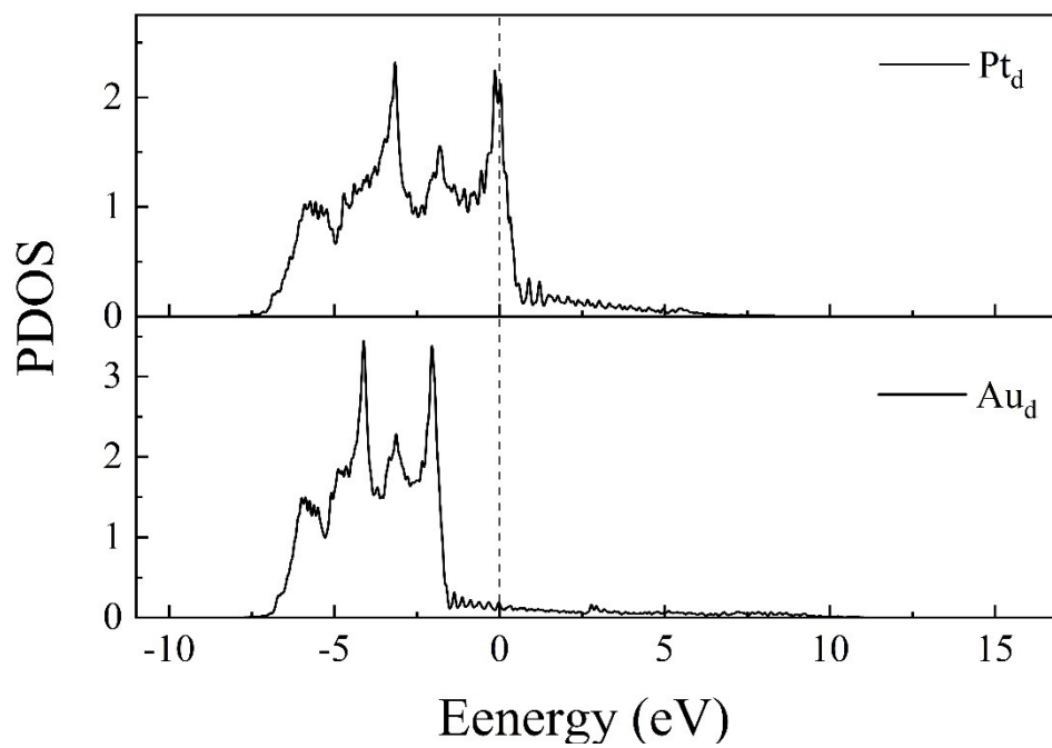
Fig. S1 PDOS diagram of d-band for Pt and Au.
