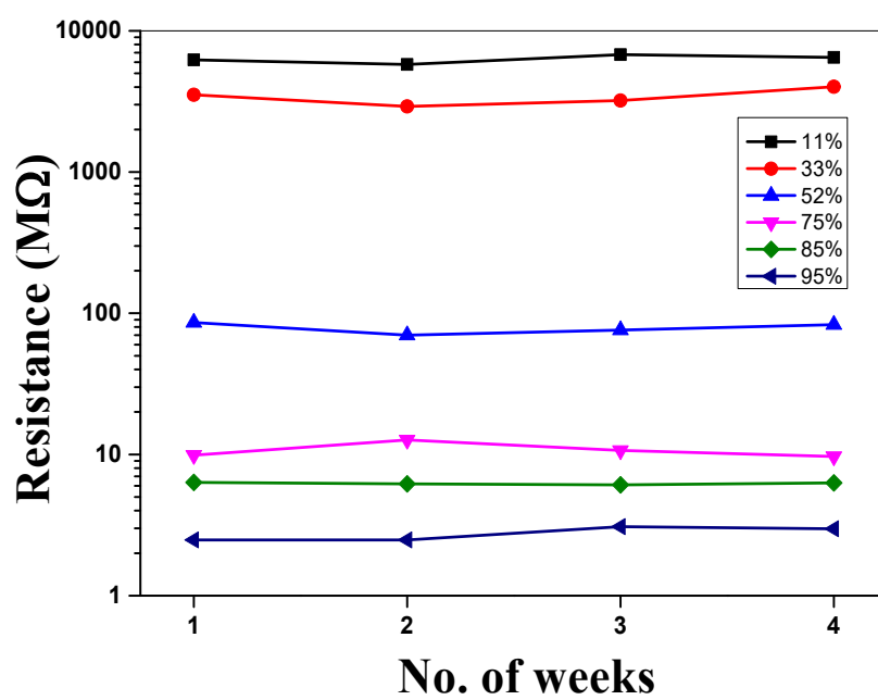
Fig. S2. Long term stability of the TiO 2 -MWCNTs composite based sensor.
