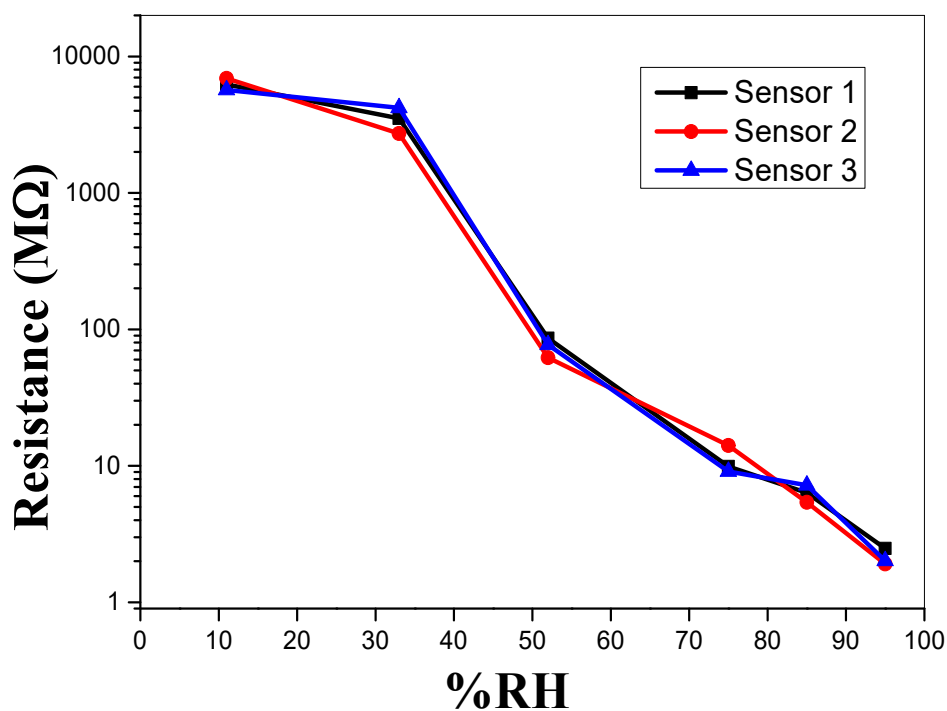
Fig. S1. The responses of the 3 composite sensors with respect to relative humidity.
