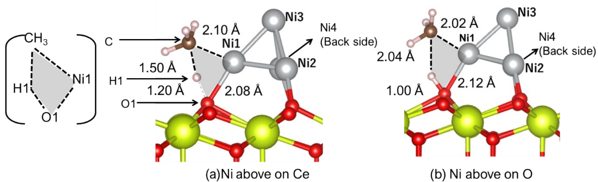
Figure S1 □ Dissociating methane and Ni clusters in the transition state (TS).
