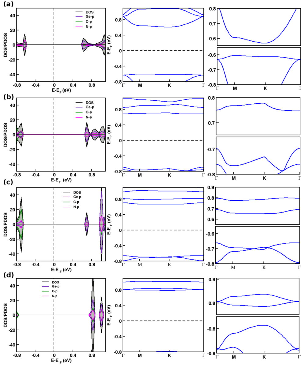
Figure S2: Zoomed-in views of N-passivated g-GeC meshes of varying sizes: (a) 5 \times 5 , (b) 6 \times 6 , (c) 7 \times 7 , and (d) 8 \times 8 , demonstrating the K-dependence of the electronic bands.
