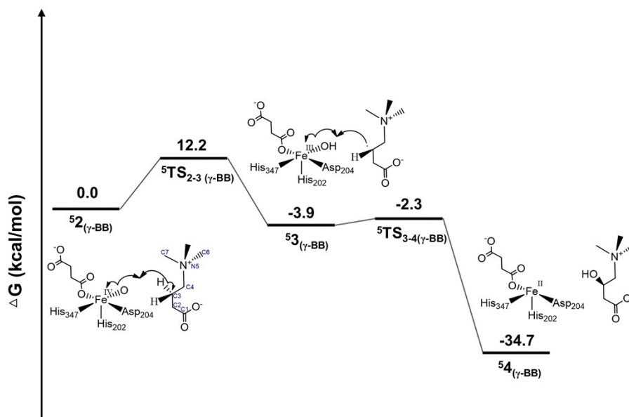
Figure S8. Free energy profile of the BBOX-catalysed \gamma -BB process in the quintet spin state.
