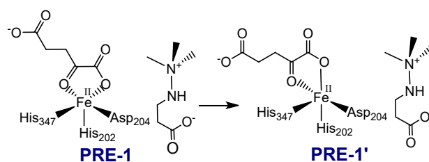
Scheme S2. A possible pathway of \text{Fe}^{\text{IV}}=\text{O} group isomerization in BBOX. 2OG rotates before \text{O}_2 binding.
