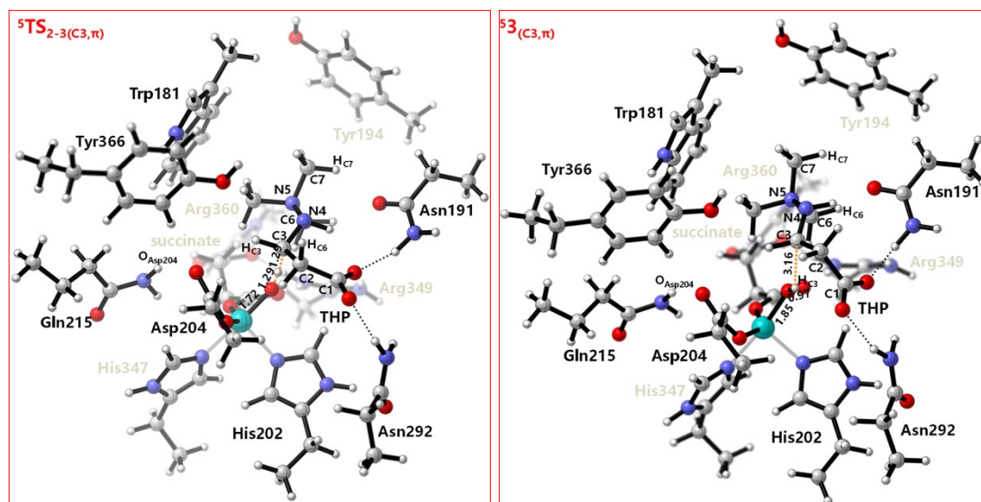
Figure S2. The optimized structures of the stationary points along the reaction process of the THP hydroxylation and rearrangement catalysed by BBOX. Bond lengths are given in Å.
