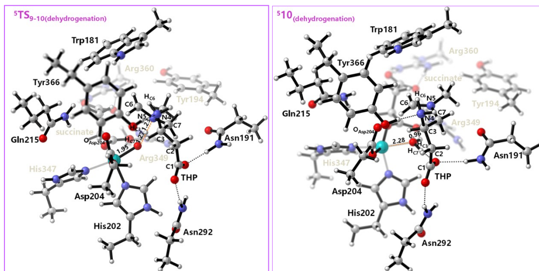
Figure S2. The optimized structures of the stationary points along the reaction process of the THP hydroxylation and rearrangement catalysed by BBOX. Bond lengths are given in Å.
