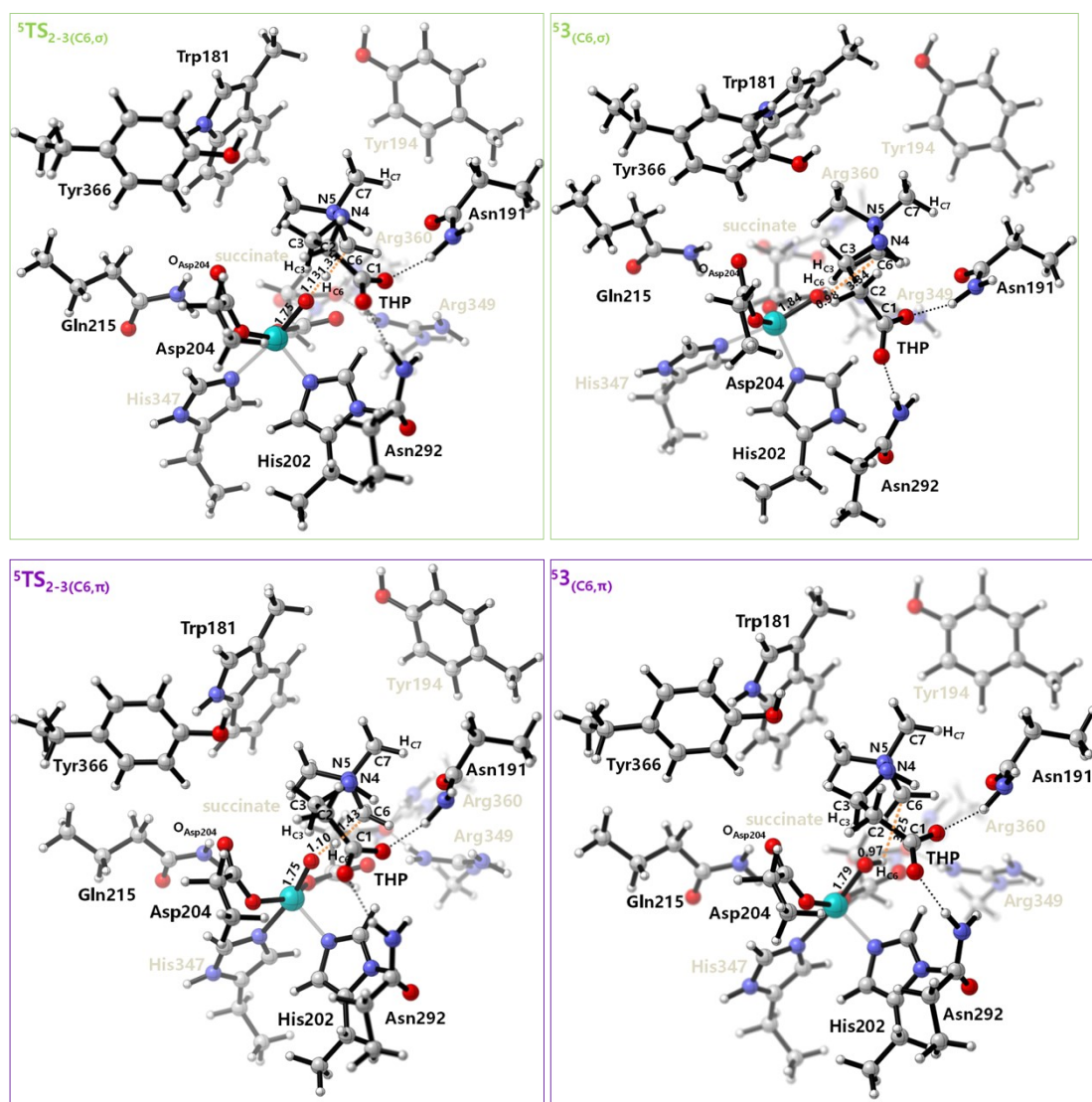
Figure S3. The optimized structures of the stationary points along the reaction process of other possible pathways to proceed the first hydrogen atom abstraction from THP catalysed by BBOX. Bond lengths are given in Å.
