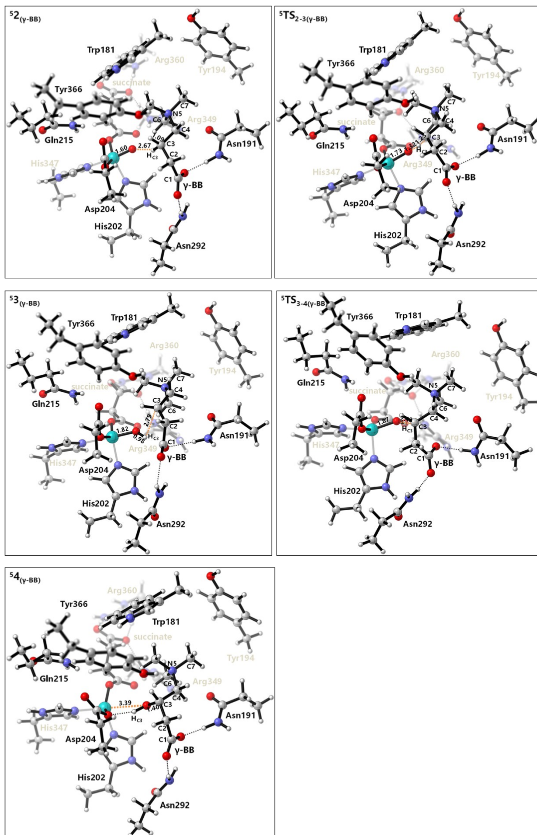
Figure S9. The optimized structures of the stationary points along the reaction process of the \gamma -BB hydroxylation catalysed by BBOX. Bond lengths are given in Å.
