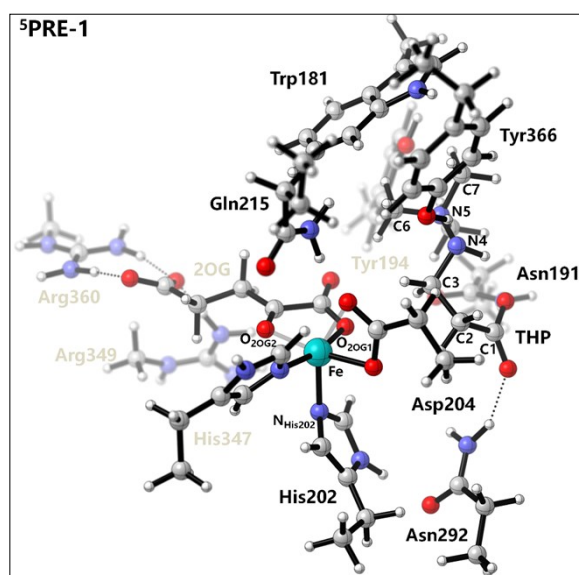
Figure S5. The optimized geometry of ^5\text{PRE-1} in the quintet spin state of BBOX.
