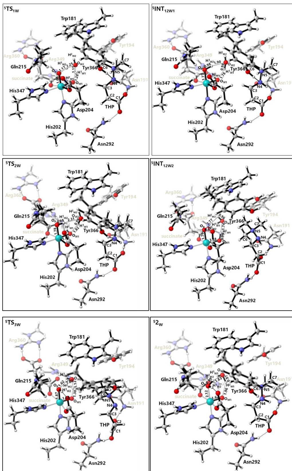
Figure S1. The optimized structures of the stationary points along the \text{Fe}^{\text{IV}}=\text{O} group isomerization process in the quintet spin state of BBOX. Bond lengths are given in Å.
