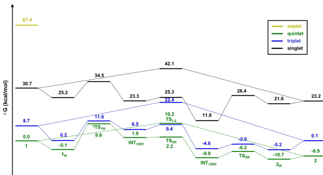
Figure S7. Free energy profile of the Fe IV =O group isomerization processes in BBOX in different spin states.
