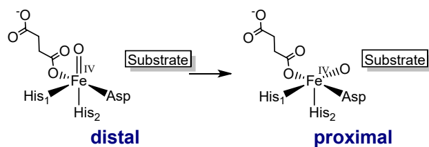
Scheme S1. \text{Fe}^{\text{IV}}=\text{O} species transition from distal to proximal type conformation.
