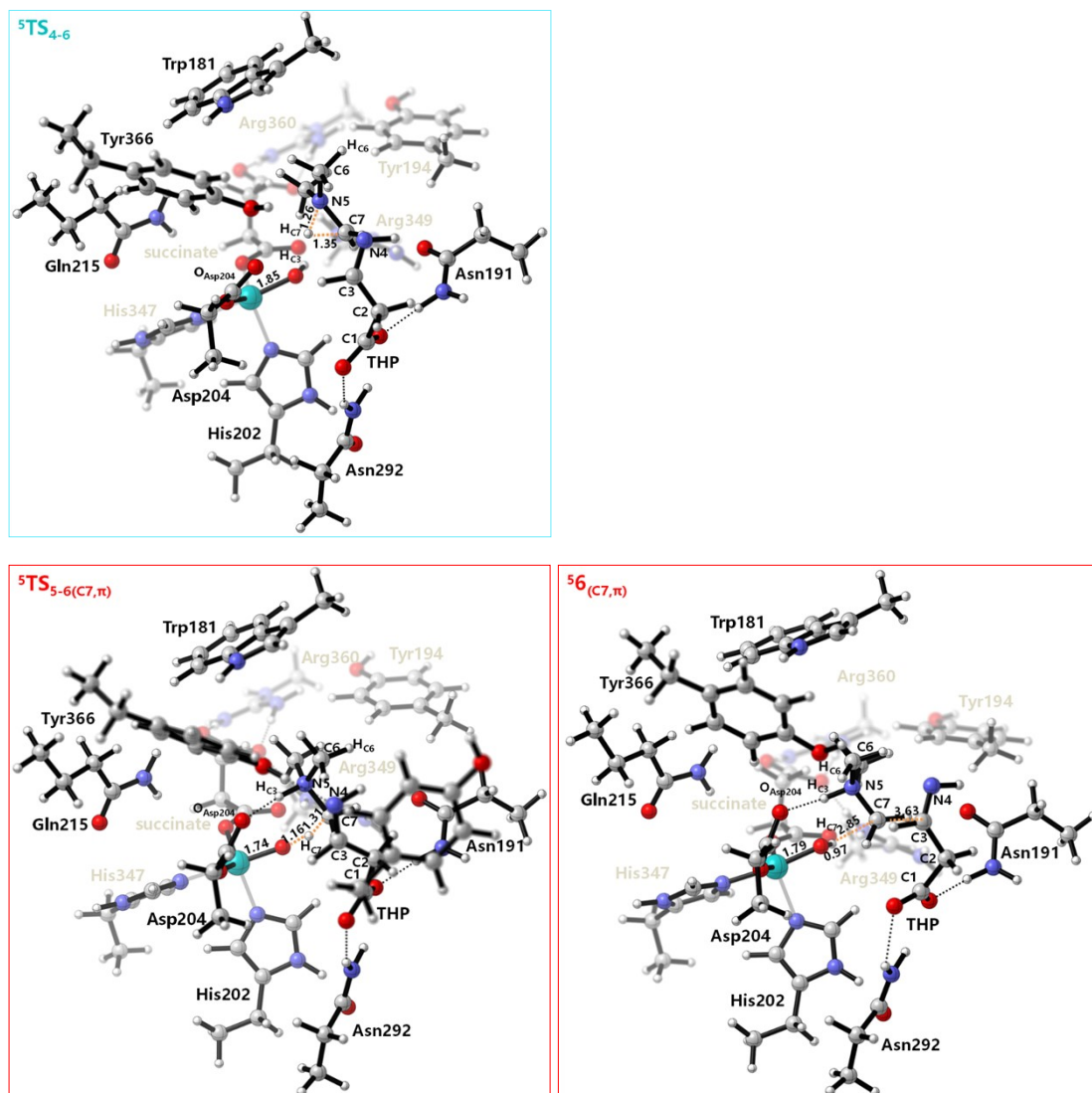
Figure S4. The optimized structures of the stationary points along the reaction process of other possible pathways to generate the C7 methylene radical species in BBOX. Bond lengths are given in Å.
