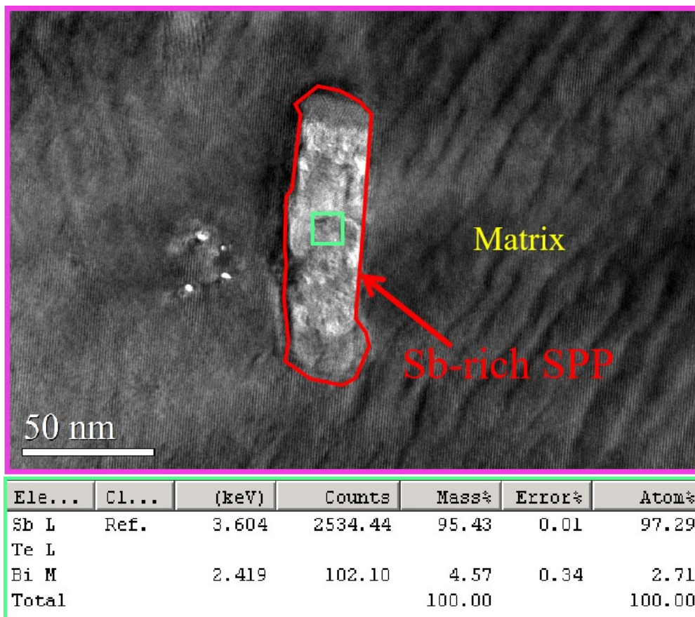
Fig. S2 The energy dispersive spectrometer (EDS) results of elongated Sb-rich SPP.
