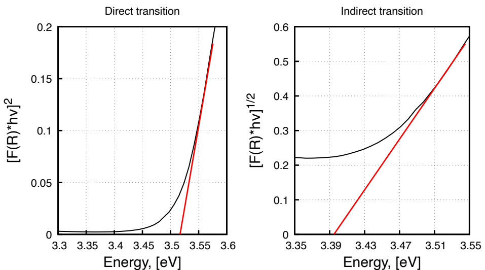
Mn-DAu Tauc plot
