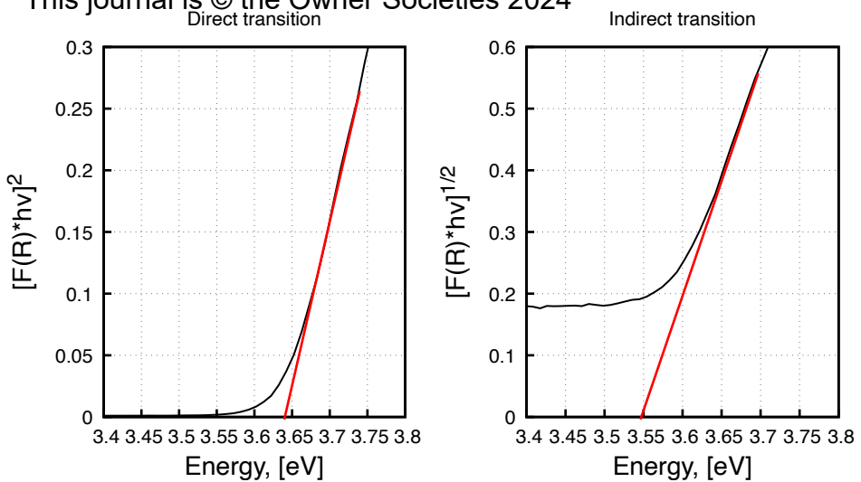
Zn-DAu Tauc plot
