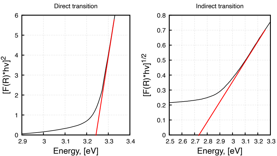
Ni-DAu Tauc plot
