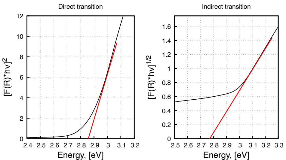
Mn-DAu Tauc plot
