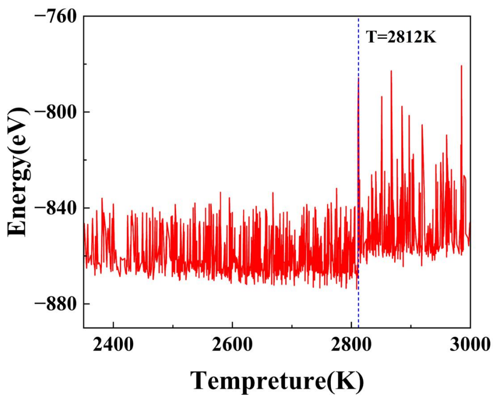
Fig. S1 Variation of structure and energy with temperature.
