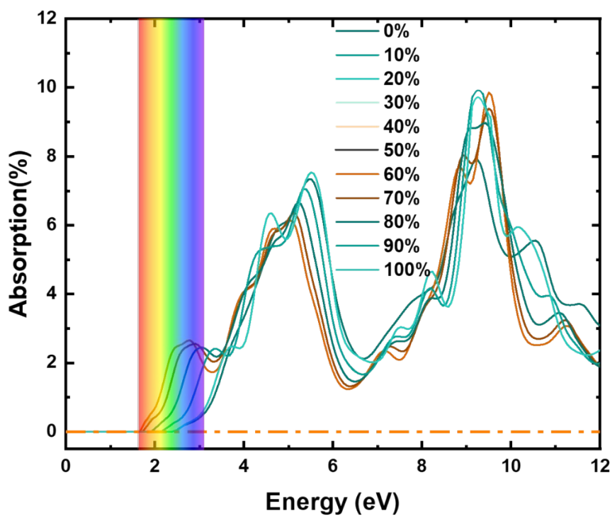
Fig. S1 Optical absorption spectra of the intermediate states between Ferroelectric Phase I and Ferroelectric Phase II, ranging from 0% to 100%. The visible light region is highlighted with a rainbow-colored background.
