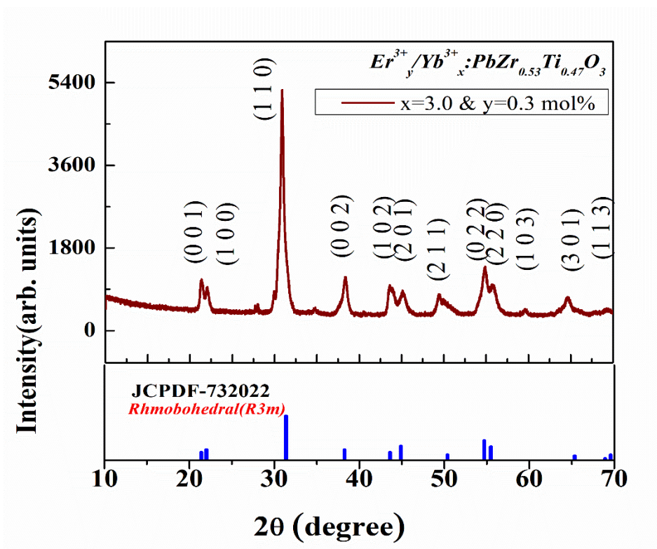
ESI:S1: Powder XRD pattern of Er^{3+}/Yb^{3+}:PbZr_{0.53}Ti_{0.47}O_3 sample synthesized via low temperature assisted combustion reaction route along with their standard profile(JCPDS) data.
