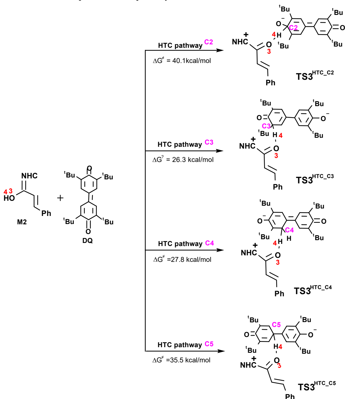
Scheme S1. Other possible HTC pathways.
