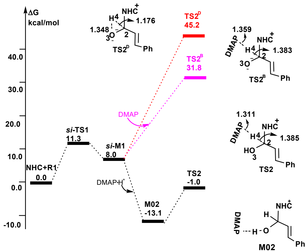
Fig. S3 Possible pathways for [1,2]-proton transfer. Energies and distances are given in kcal/mol and Å, respectively.
