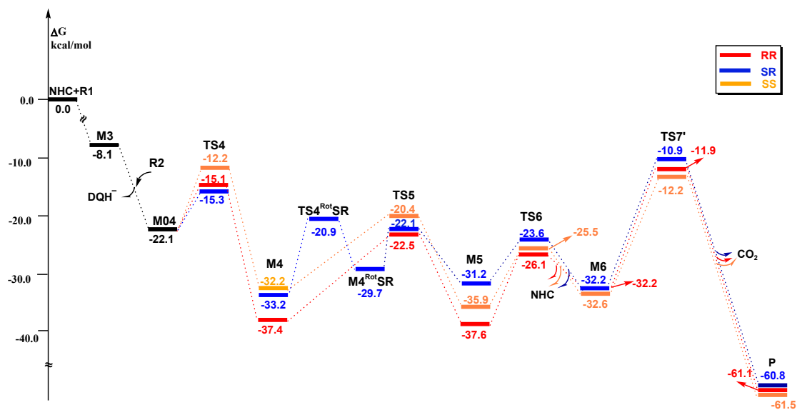
Fig. S4 Unfavorable pathways for the reaction of M3 and R2. Energies are given in kcal/mol.
