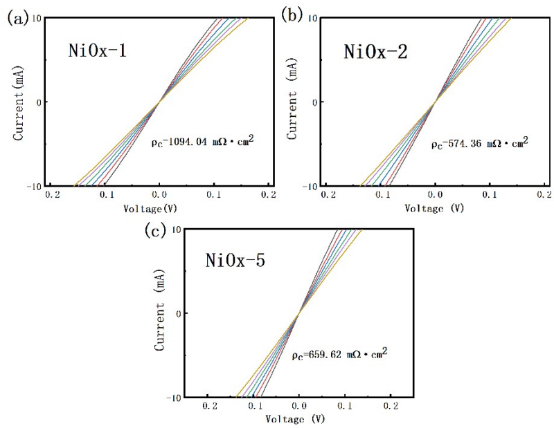
Fig S4 (a)-(d). Contact resistivity test for NiOx-1, NiOx-2, NiOx-5
