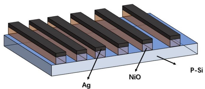
Fig.S3. The structures of the test of the contact resistance
