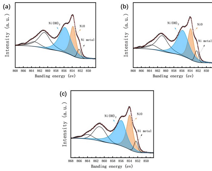
FigS6(a)-(c) XPS test of NiOx-1A, NiOx-2A, NiOx-5A
