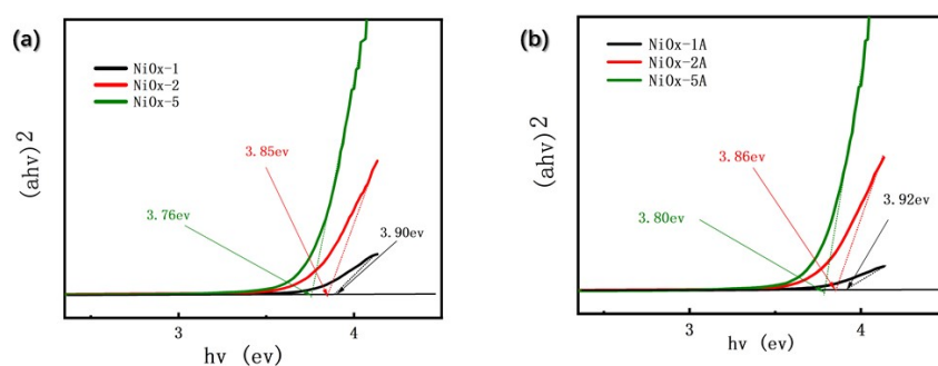
Fig.S2. The bandgap widths of different NiOx films
