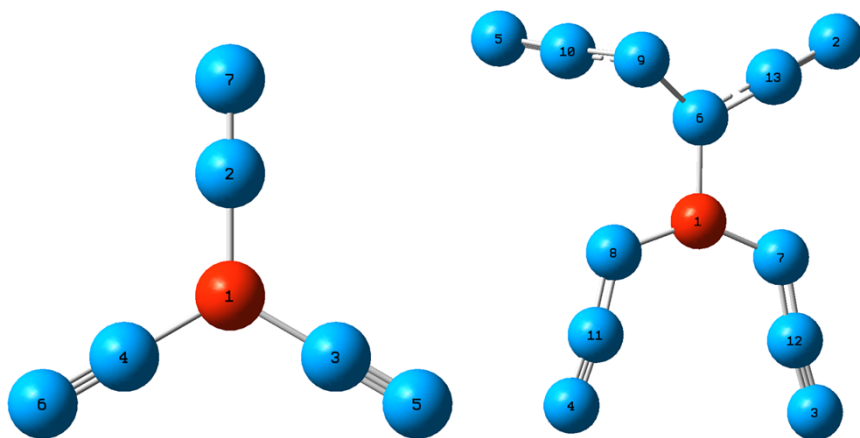
Fig. S1 The labels of B and N atom in lowest-energy structure of \text{BN}_6^+ and \text{BN}_{12}^+ cluster.
