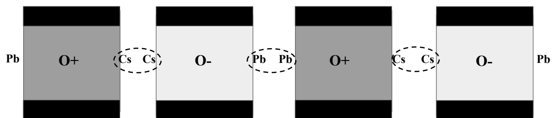
Figure S1: Ground state of the 1D arrangement
