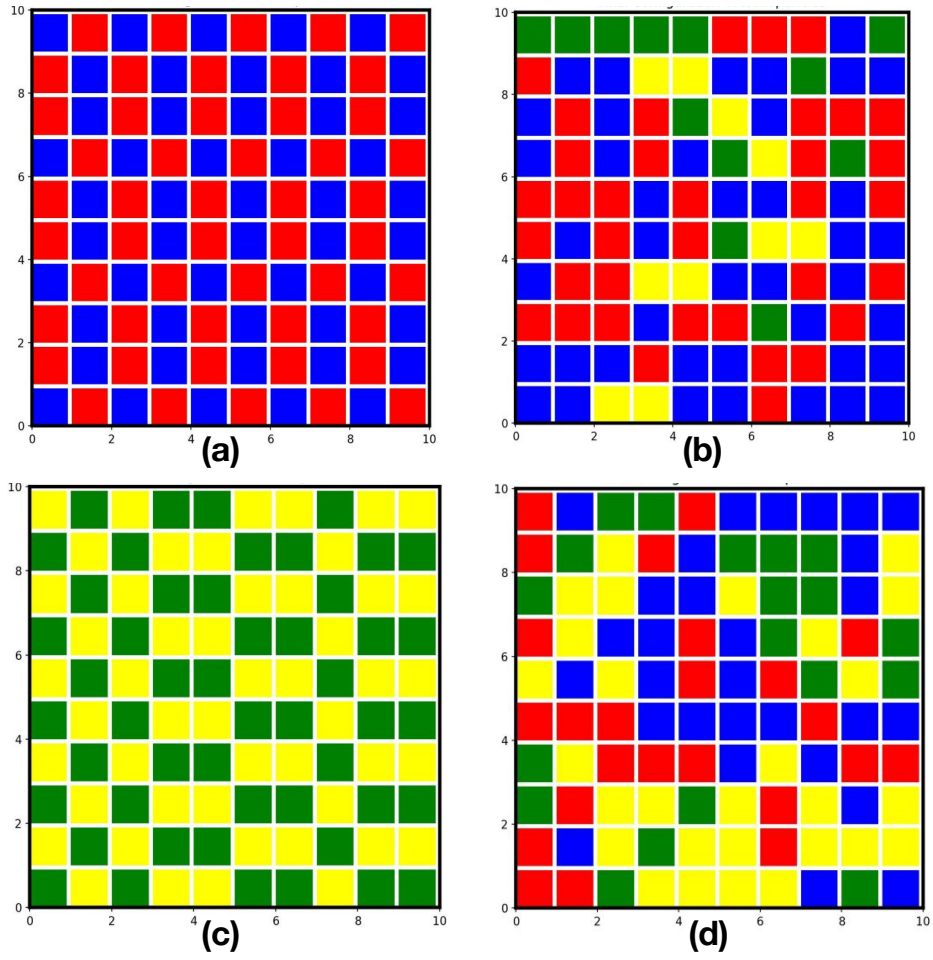
Figure S2: Snapshot of 2D N \times N arrangement for N=10
