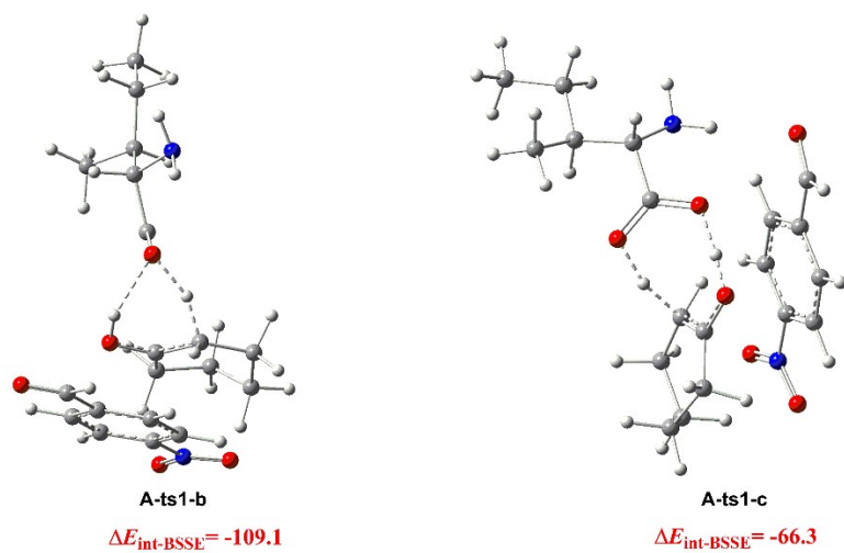
Figure S1. The interaction energy with BSSE correction for A-ts1-b and A-ts1-c.
