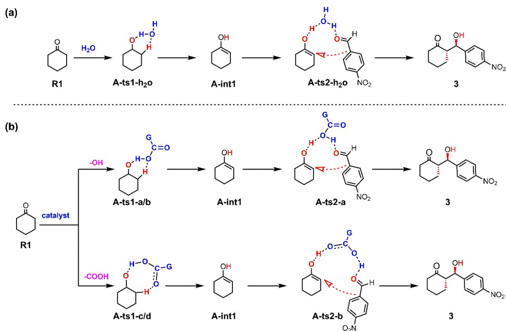
Scheme S1. The reaction mechanism involved \text{H}_2\text{O} and catalyst.
