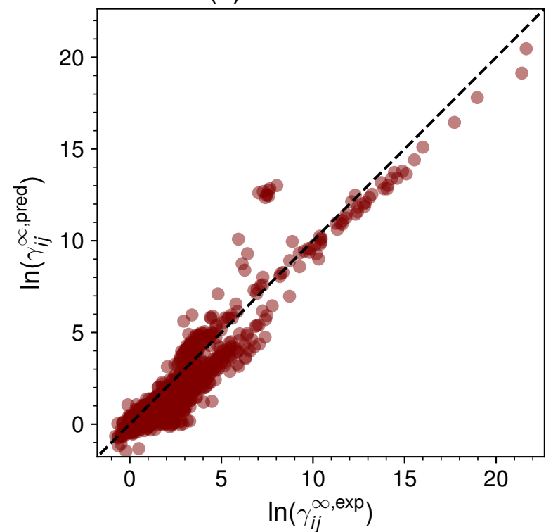
(c) COSMO-SAC
