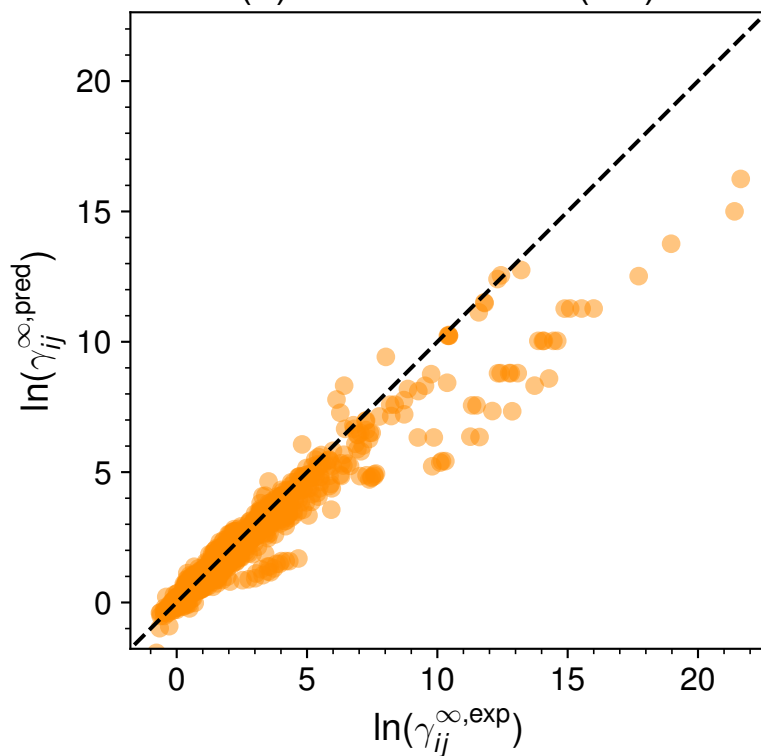
(b) Mod. UNIFAC (Do)
