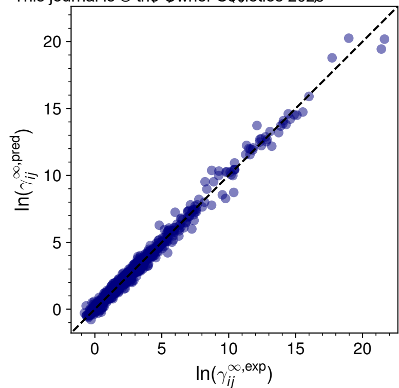
(a) SBM ( r = 0.93 )
