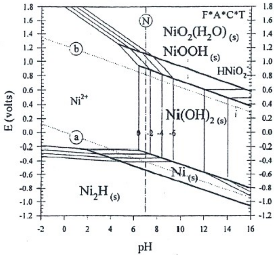
Fig S2. The Pourbaix Diagram for nickel (Ni) through experiment 1 .
