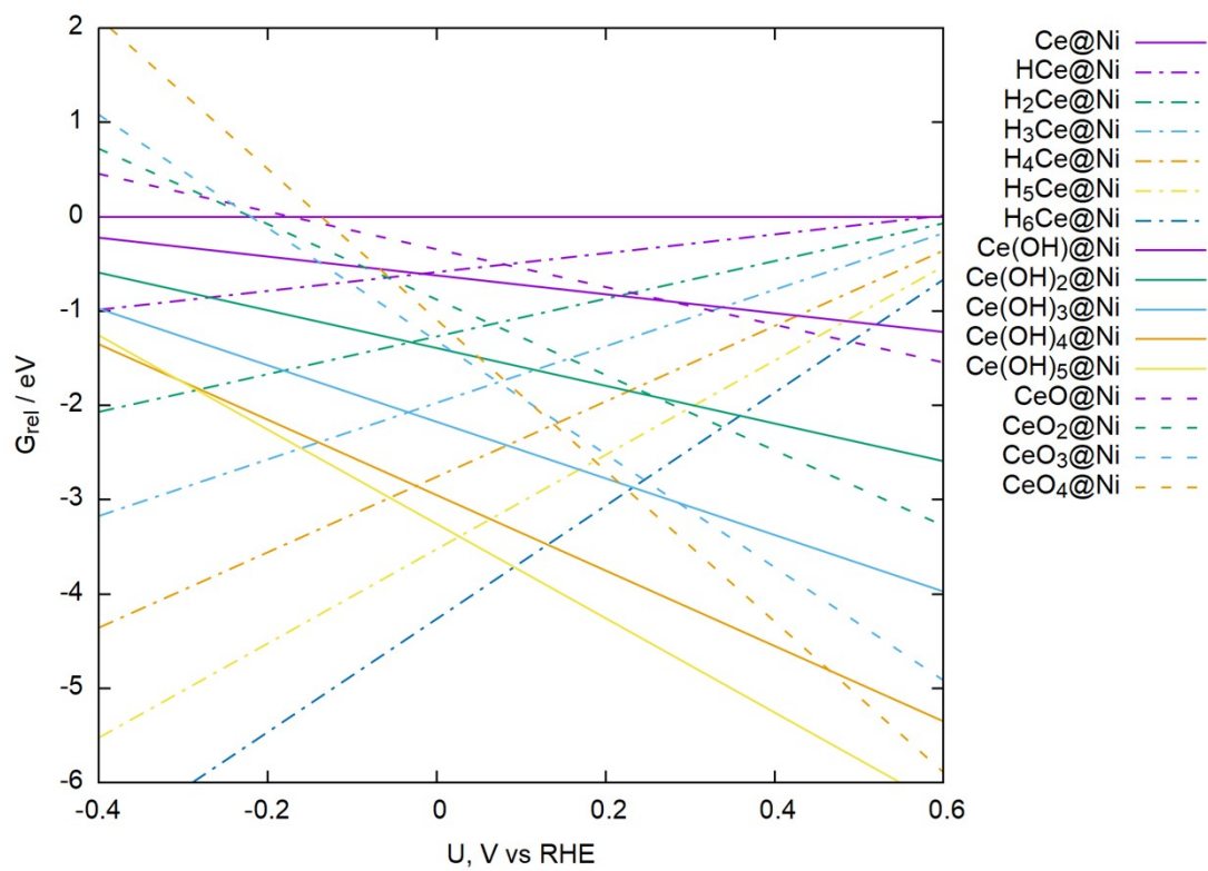
Fig S4. The Pourbaix diagram illustrating surface reactions of monodisperse Ce@Ni at pH = 0.
