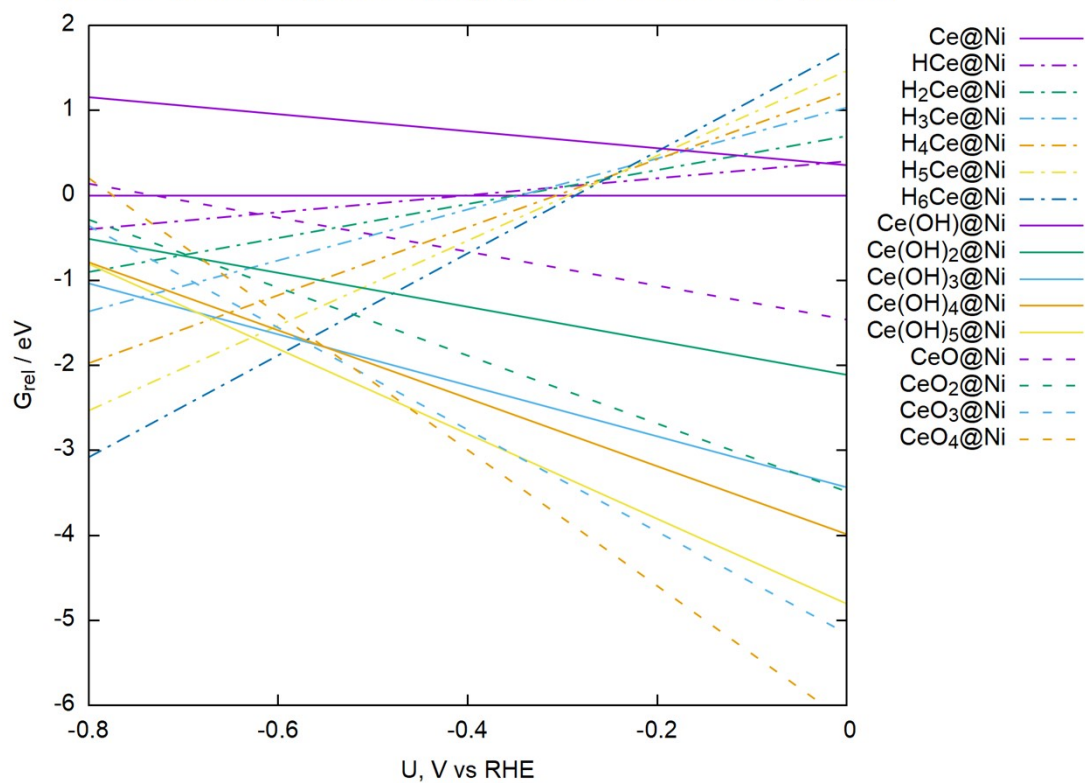
Fig S5. The Pourbaix diagram illustrating surface reactions of monodisperse Ce@Ni at pH = 14.
