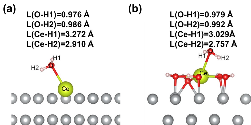
Fig S6. O-H bond length and Ce-H distance for adsorbed H 2 O on (a) Ce@Ni and (b) Ce(OH) 5 @Ni surfaces.
