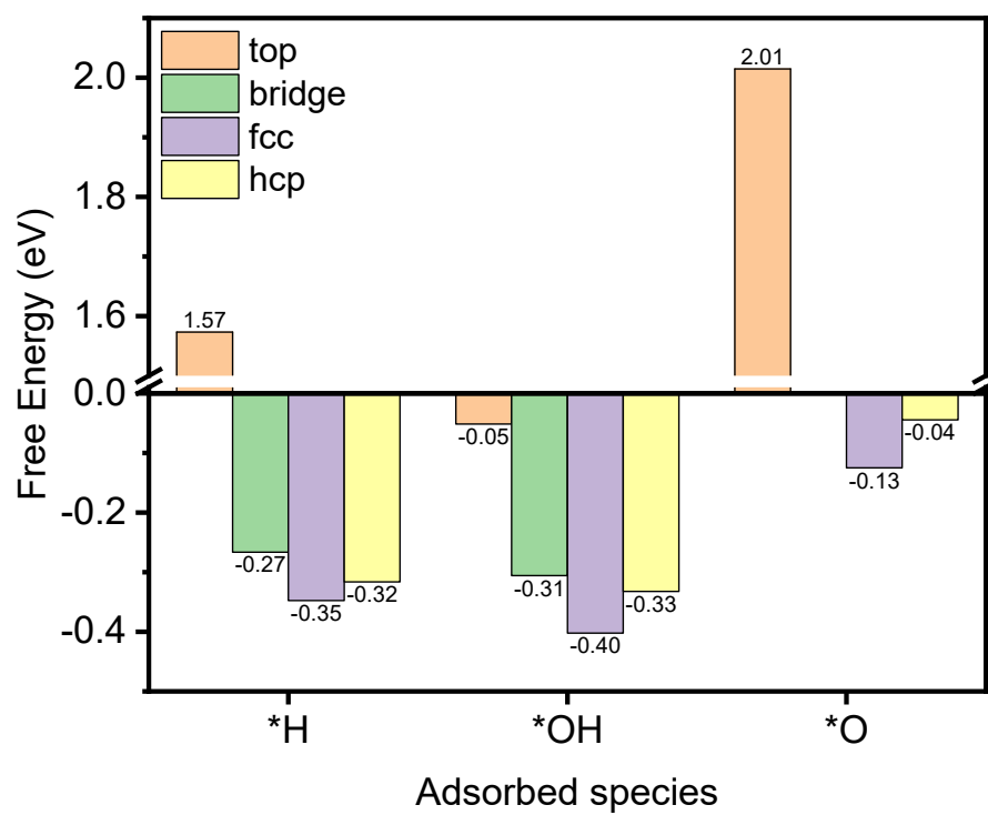
Fig S1. The Free energy of *H, *OH, and *O on the surface of Ce@Ni.
