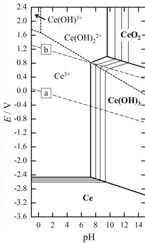
Fig S3. The Pourbaix Diagram for cerium (Ce) through experiment 1,2 .
