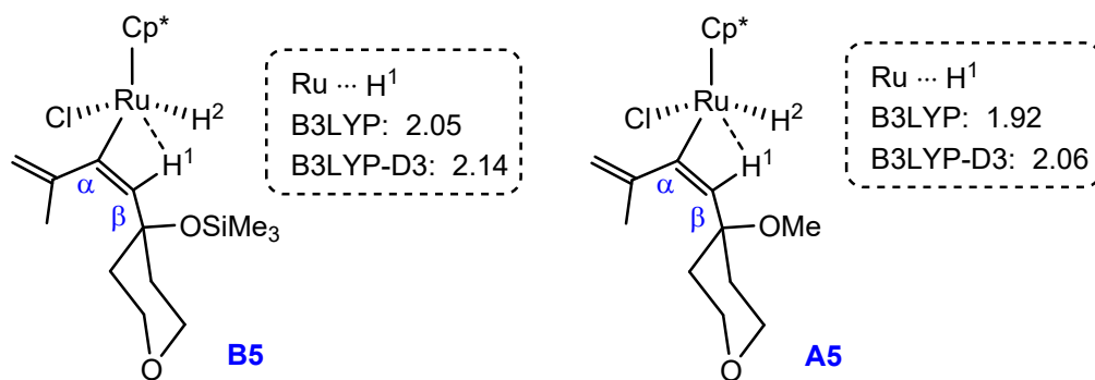
Figure S6. Calculated the Ru...H 1 distances in A5 and B5 using B3LYP and B3LYP-D3 methods, respectively.
