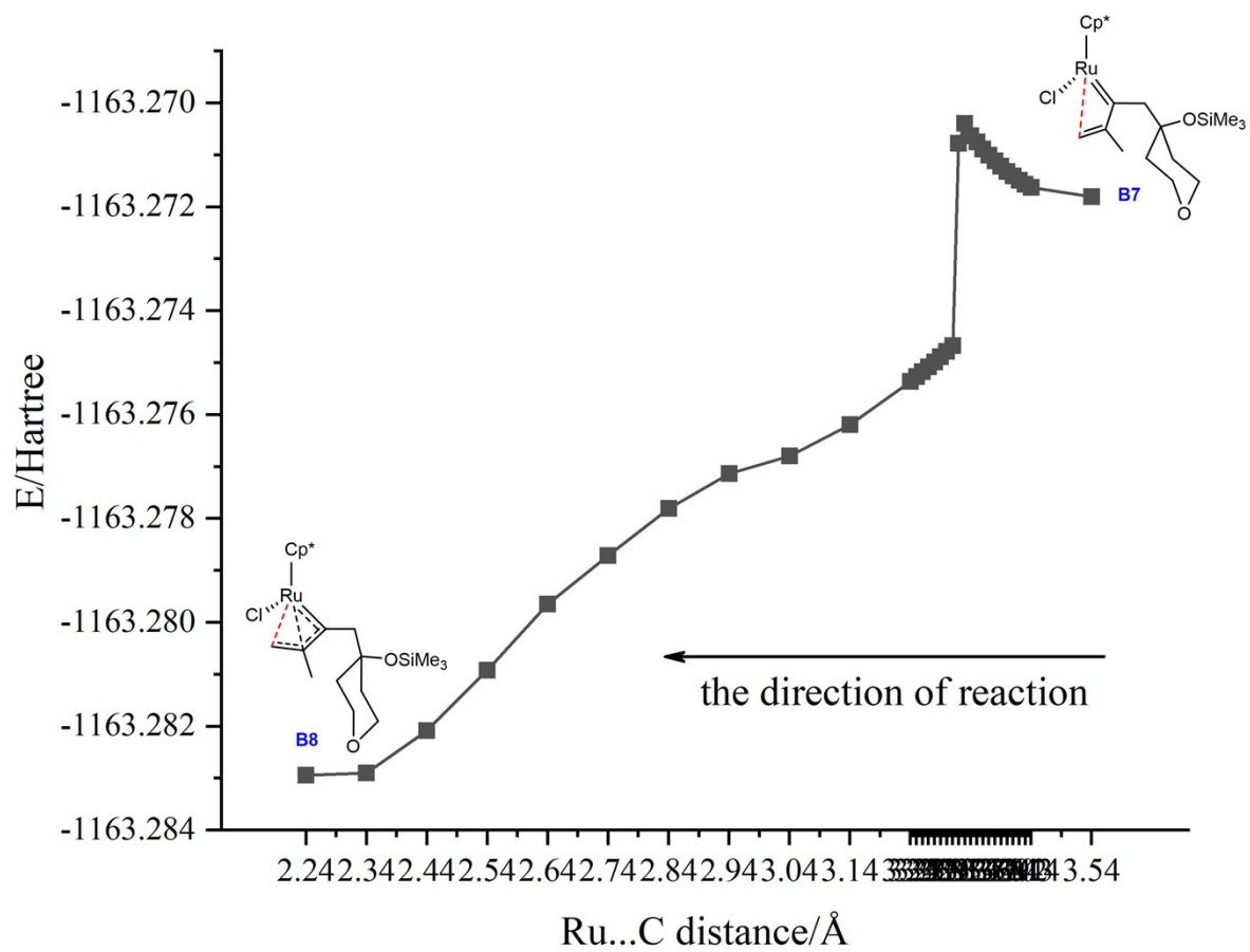
Figure S3. Scan of r(\text{Ru}\cdots\text{C}_{\text{sp}^2}) vs electronic energy E from complex B7 to intermediate B8 in Reaction
