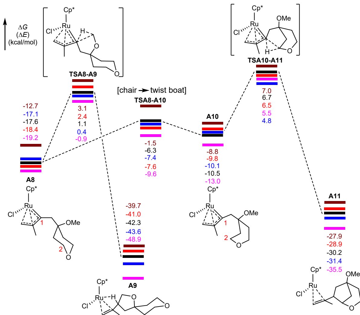
Figure S1. Calculated Gibbs free energy profile for cyclization processes in model reaction A using different computational methods. Full optimizations in dichloroethane solvent have been performed with SMD model.
