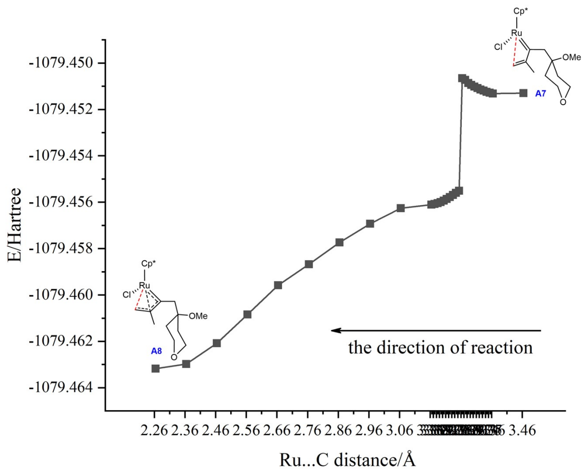
Figure S2. Scan of r(\text{Ru}\cdots\text{C}_{\text{sp}2}) vs electronic energy E from complex A7 to intermediate A8 in Reaction
