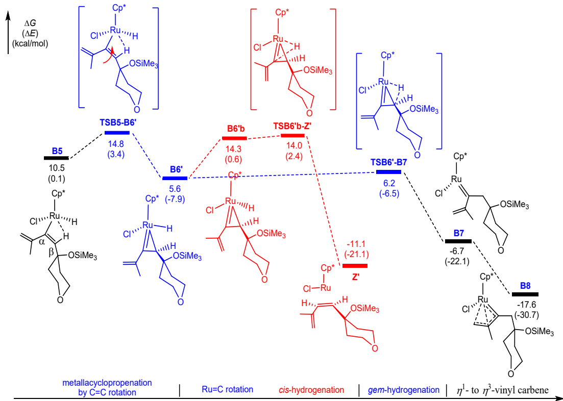
Figure S5. Calculated Gibbs energy profiles for gem -hydrogenation and cis -hydrogenation of the substrate 1,3-ene from another metallacyclopropane intermediate B6' mediated by [\text{Cp}^*\text{RuCl}]_4 in Reaction B.
