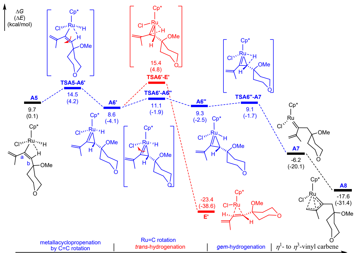
Figure S4. Calculated Gibbs energy profiles for gem -hydrogenation and trans -hydrogenation of the substrate 1,3-enyne from another metallacyclopropene intermediate A6' mediated by [\text{Cp}^*\text{RuCl}]_4 in Reaction A.
