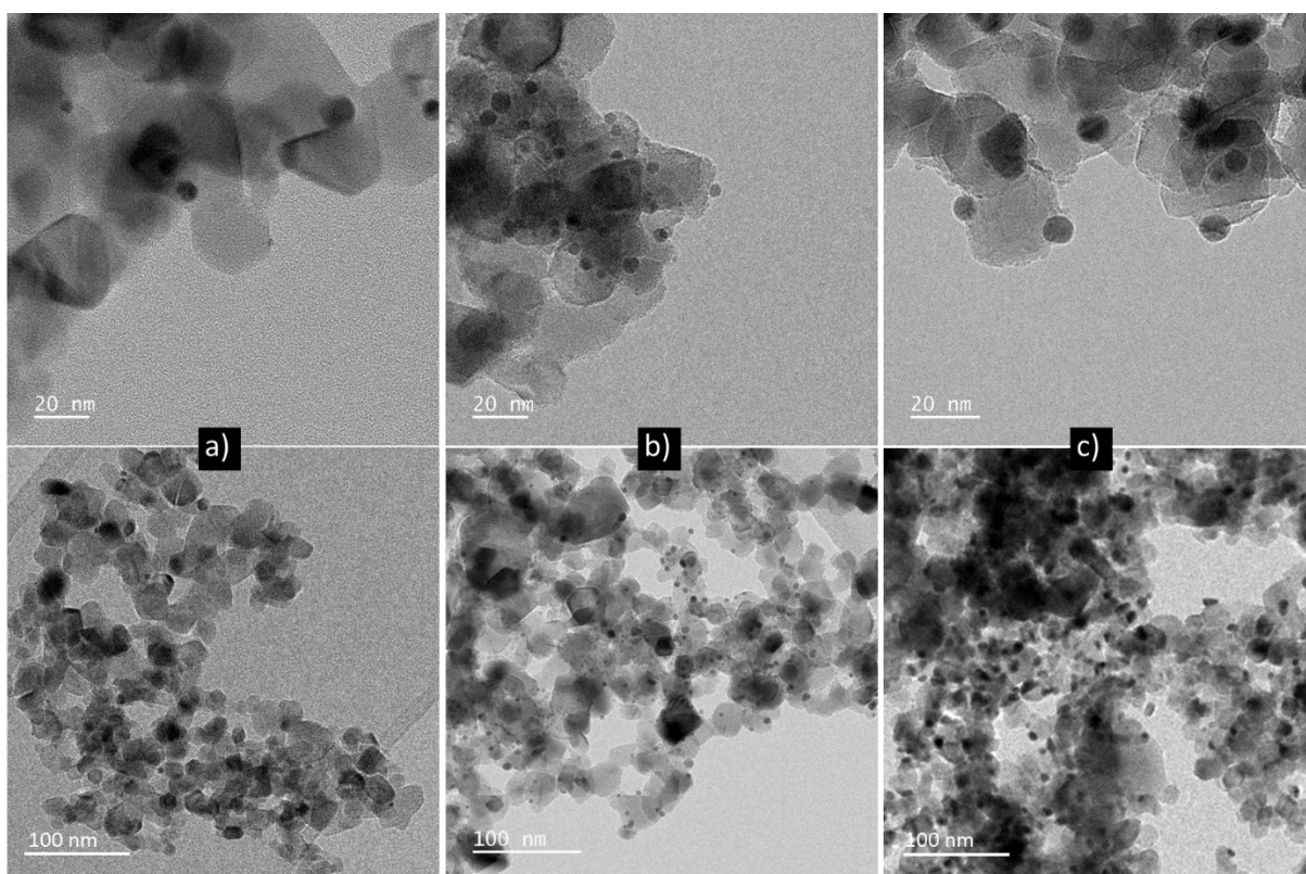
Fig. S1 TEM micrographs of P25 after: a) 0.5-h, b) 1-h and c) 1.5-h Au plasma deposition
