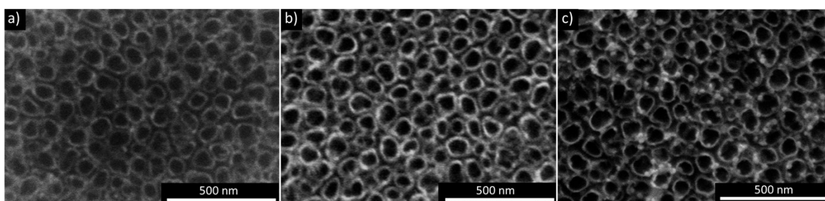
Fig. S2 SEM micrographs of TiO 2 NTs after: a) 2-min, b) 5-min and c) 10-min Au plasma deposition
