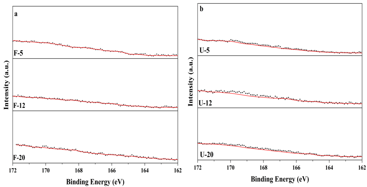
Figure. S2 XPS spectra of fresh catalysts S species, before catalytic activity test (a), after catalytic activity test (b)
