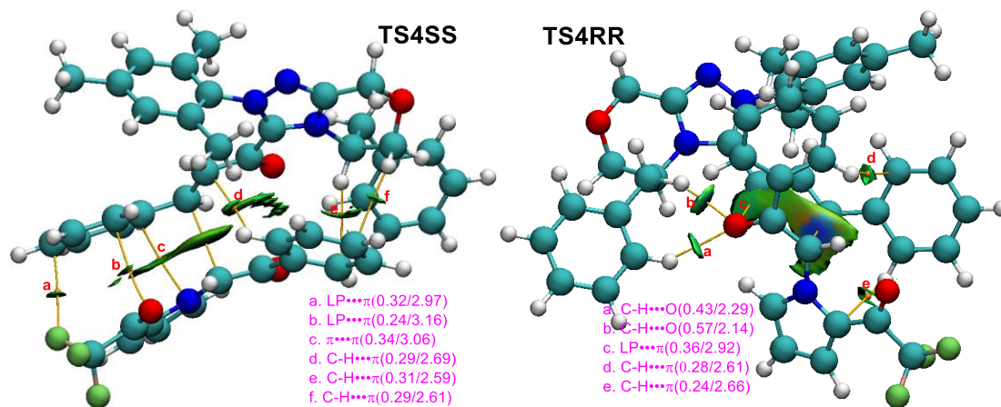
Fig. S4 NCI and AIM analyses for the enantioselective transition states of TS4SS and TS4RR (distance in Å and Laplacian of electron density \nabla^2\rho in 10^{-1} a.u.).
