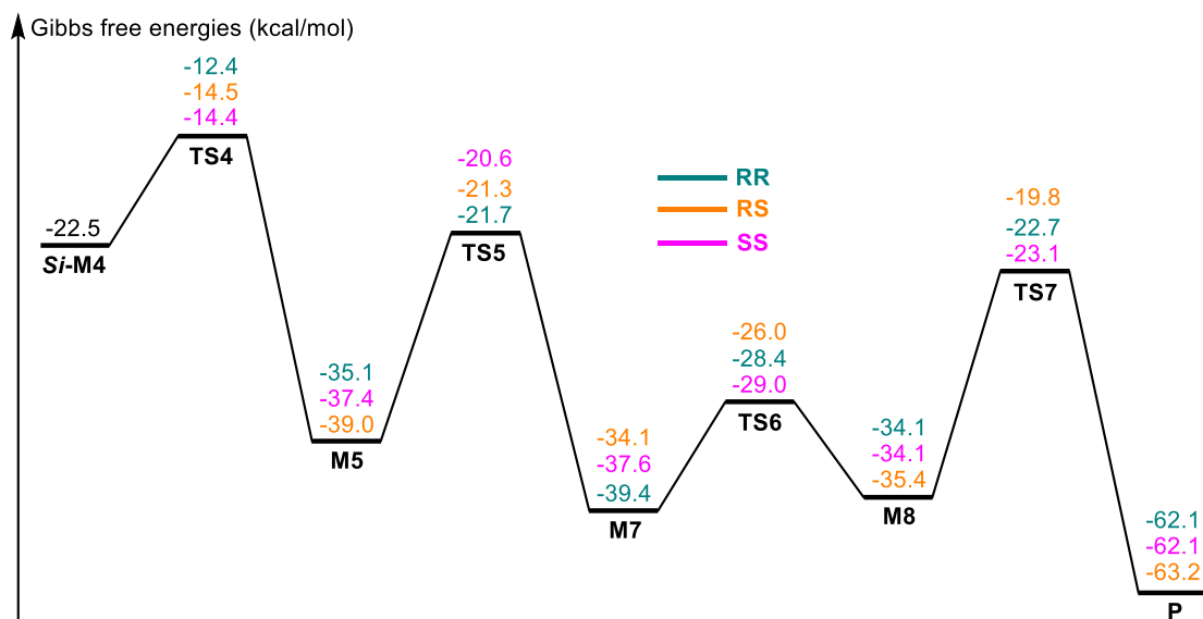
Fig. S2 Energy profile for the reaction between acyl azolium intermediate Si-M3 and R2-anion.
