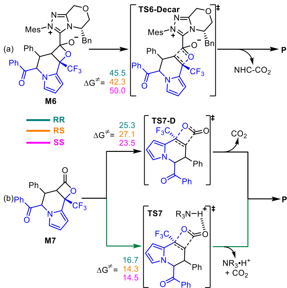
Scheme S2 Possible Pathways for Decarboxylation Process.
