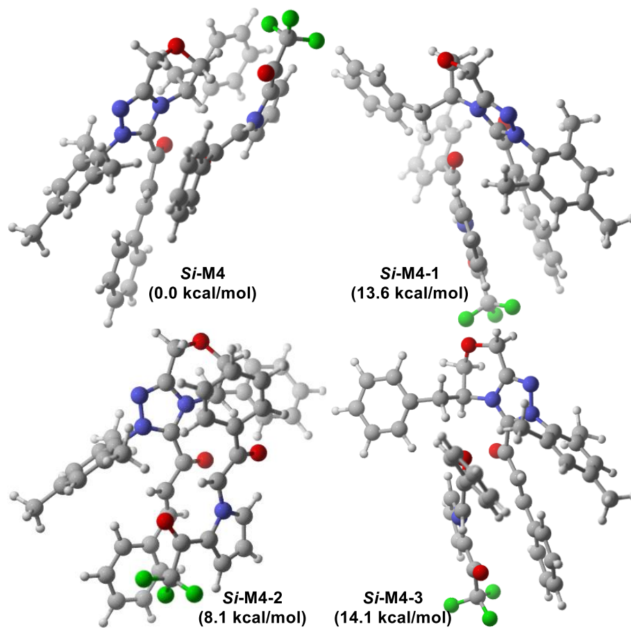
Fig. S3 Different configurations of the complex Si-M4 .
