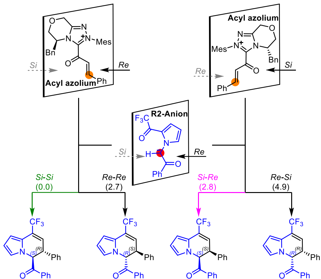
Scheme S1 Illustration of the stereoselective addition mode.
