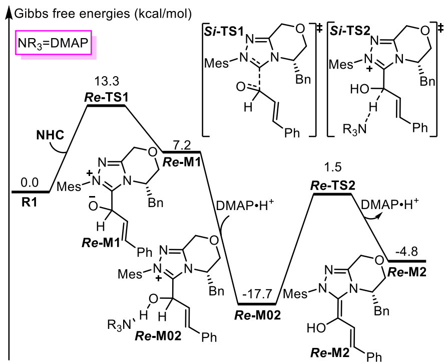
Fig. S1 Energy profile for the formation of Re -M2.
