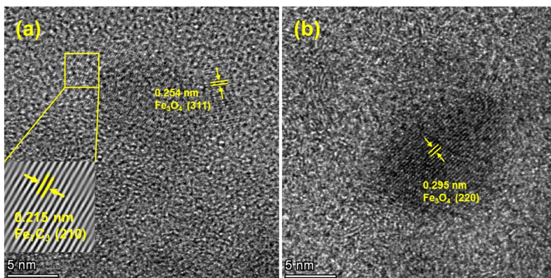
Figure S1. TEM images of the fresh (a) Fe/NC-1150 and (b) Fe/AC catalysts.
