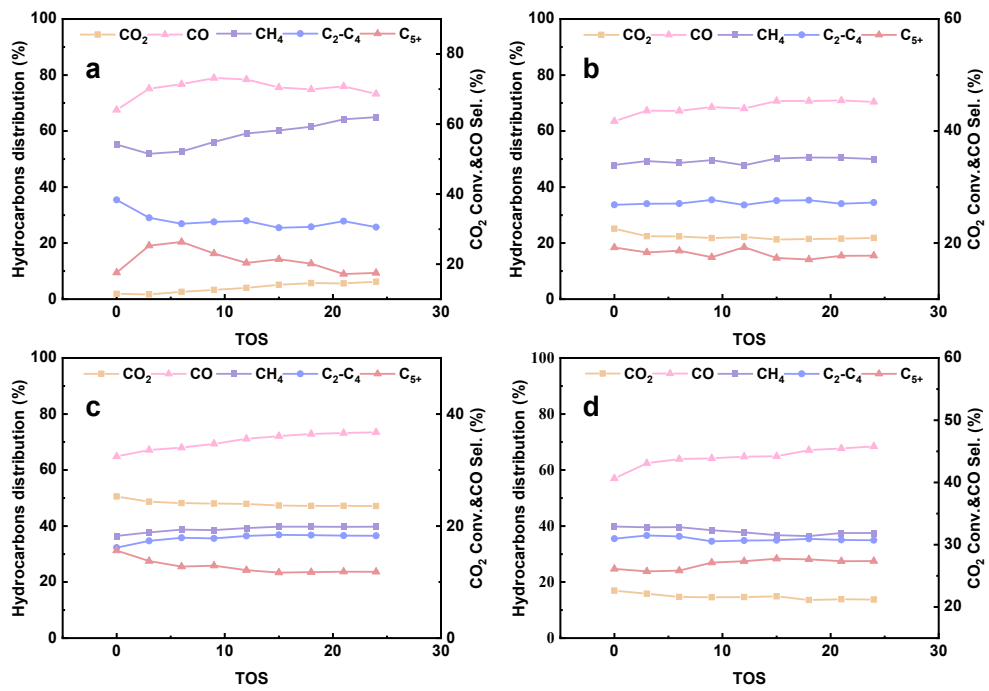
Figure S3. Catalytic performance of Fe/AC (a), Fe/NC-950 (b), Fe/NC-1050 (c) and Fe/NC-1150 (d).
