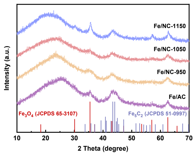
Figure S2. XRD patterns of used Fe/AC and Fe/NC-T catalysts.
