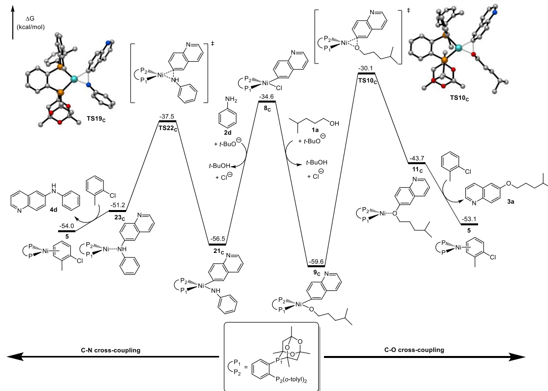
Fig. S9 Free energy profiles of Ni-catalyzed competitive arylation of the alkyl alcohol and aniline from 8c .
