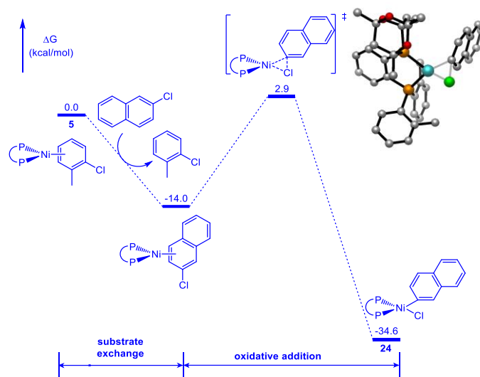
Fig. S10 Free energy profile for the formation of the intermediate 24.
