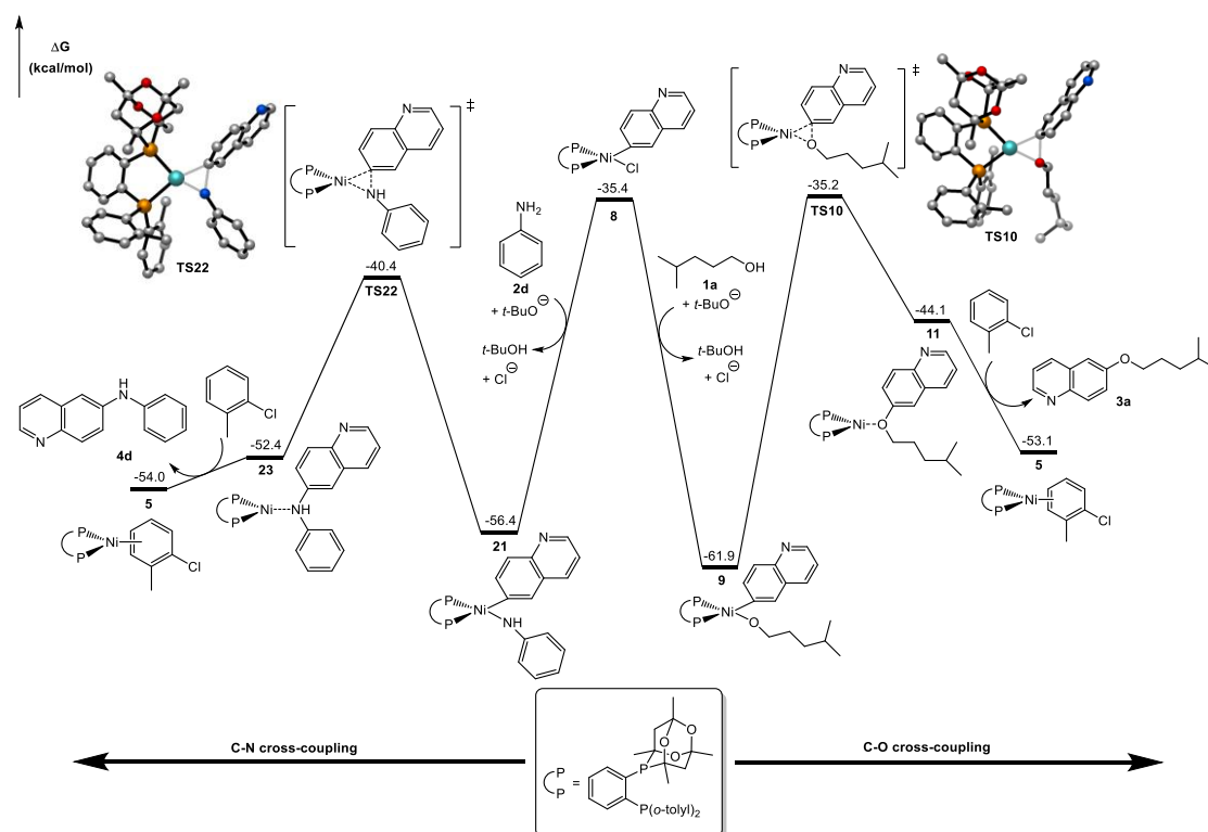
Fig. S4 Free energy profiles of Ni-catalyzed competitive arylation of the alkyl alcohol and aniline from 8 .
