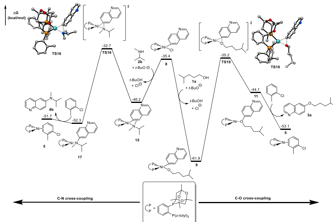
Fig. S2 Free energy profiles of Ni-catalyzed competitive arylation of the alkyl alcohol and secondary dialkylamine from 8 .
