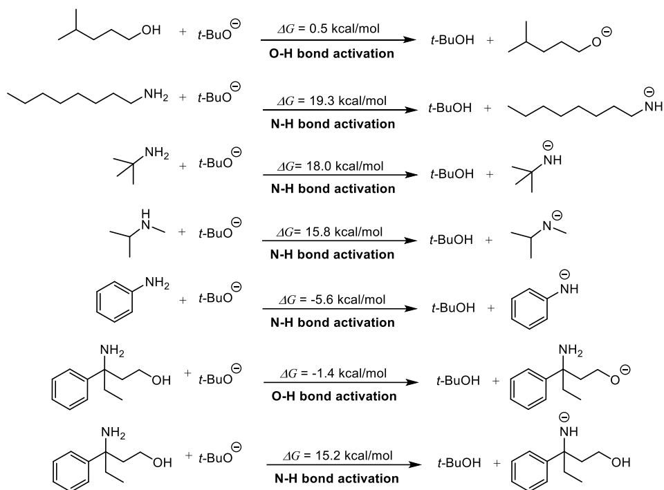
Fig. S1 Free energy changes for activation of alcohols or amines.
