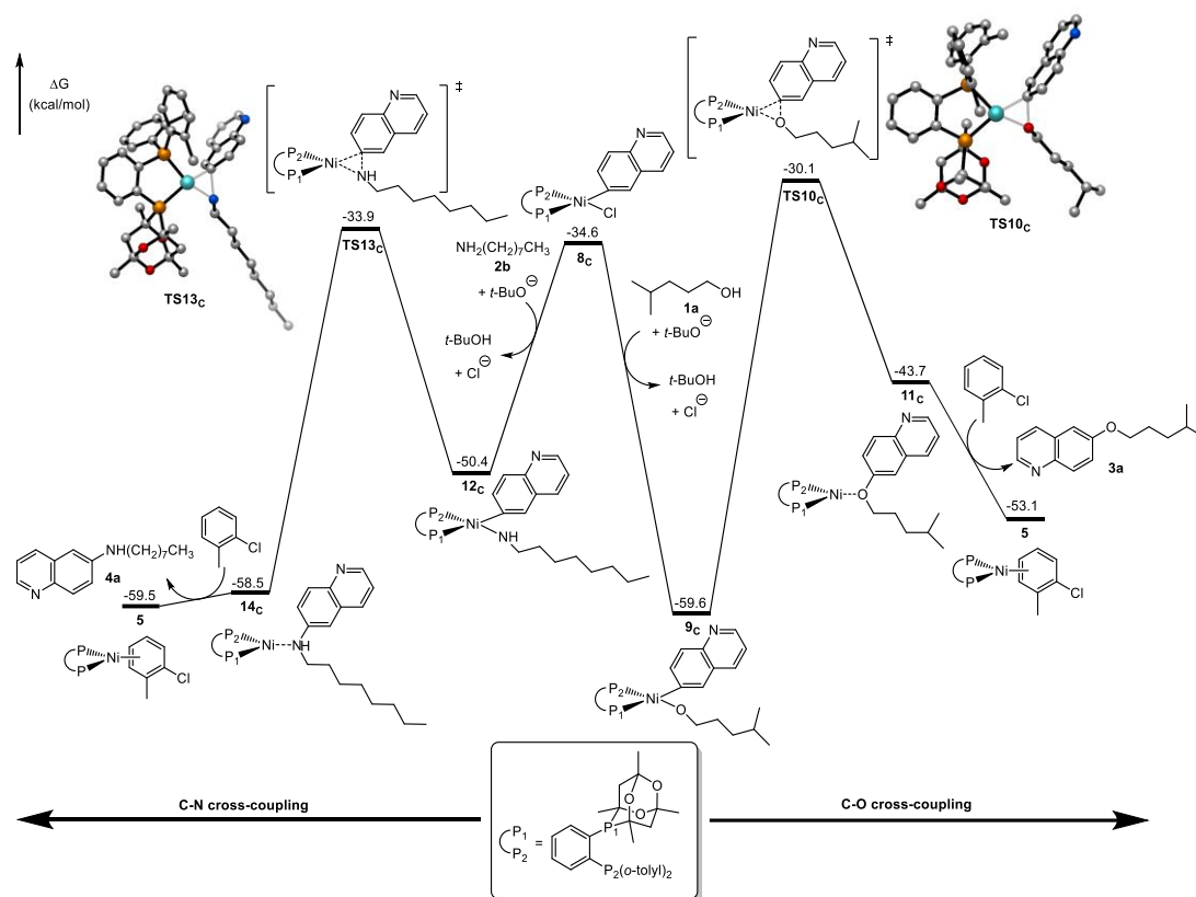
Fig. S6 Free energy profiles of Ni-catalyzed competitive arylation of the alkyl alcohol and linear alkylamine from 8c .
