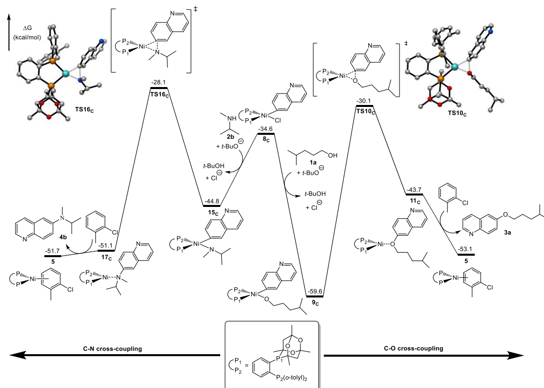
Fig. S7 Free energy profiles of Ni-catalyzed competitive arylation of the alkyl alcohol and secondary dialkylamine from 8c .
