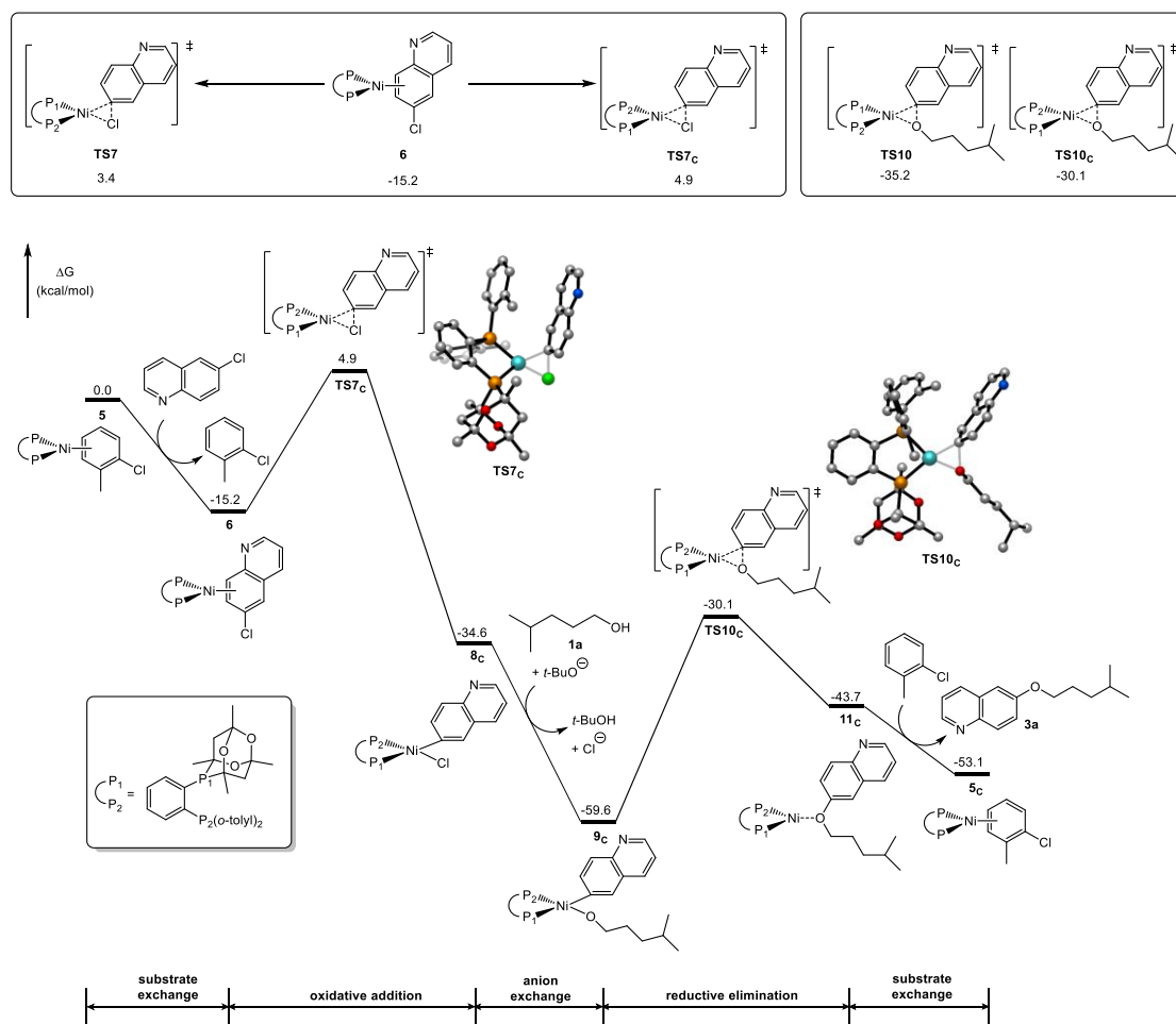
Fig. S5 Free energy profile of Ni-catalyzed C-O cross-coupling of an alcohol and heteroaryl chloride.
