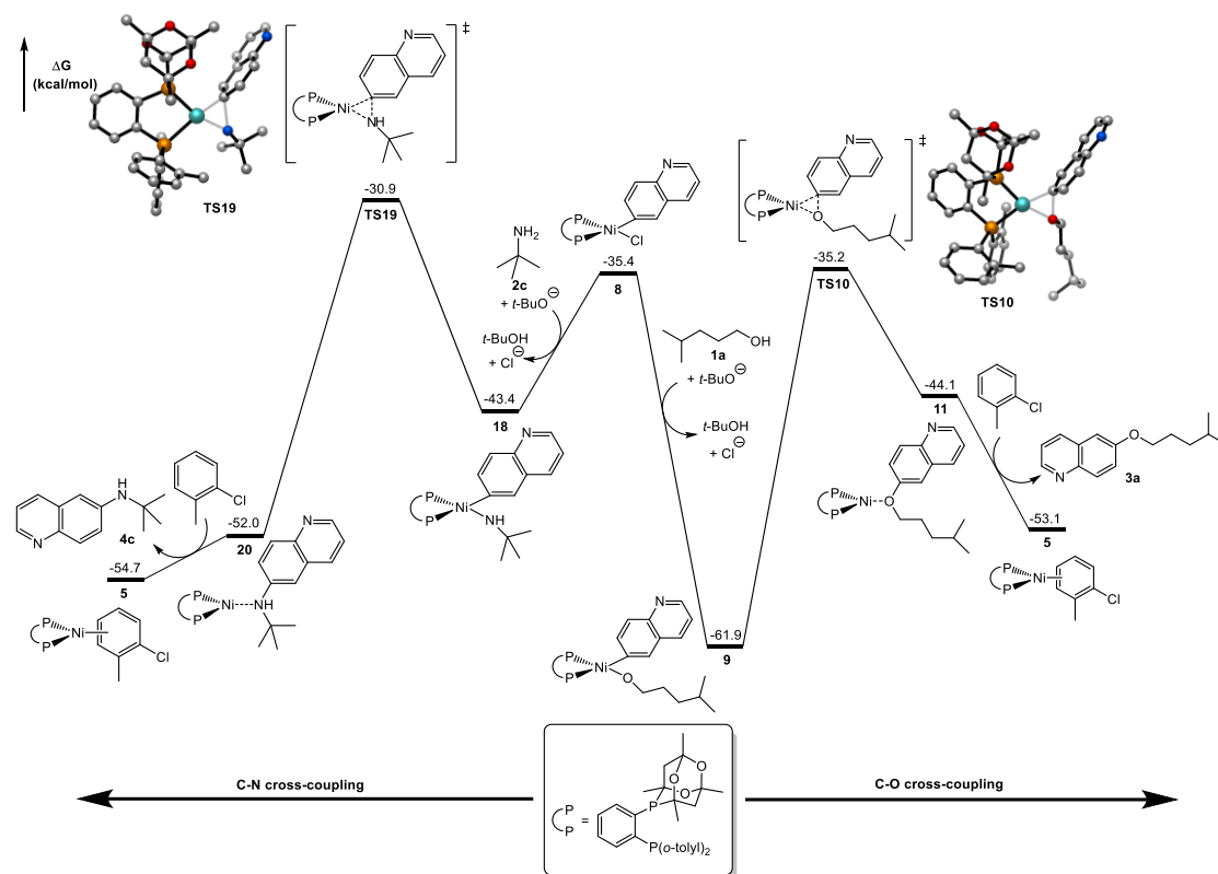
Fig. S3 Free energy profiles of Ni-catalyzed competitive arylation of the alkyl alcohol and branched primary alkylamine from 8 .
