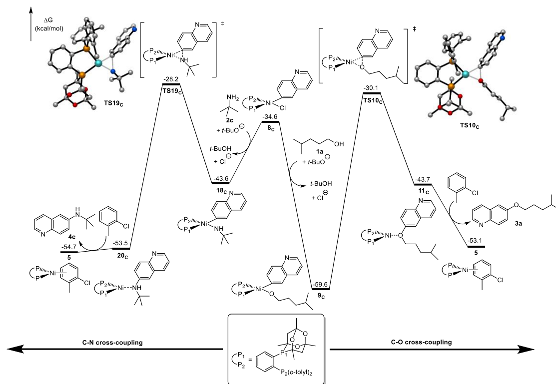
Fig. S8 Free energy profiles of Ni-catalyzed competitive arylation of the alkyl alcohol and branched primary alkylamine from 8c .
