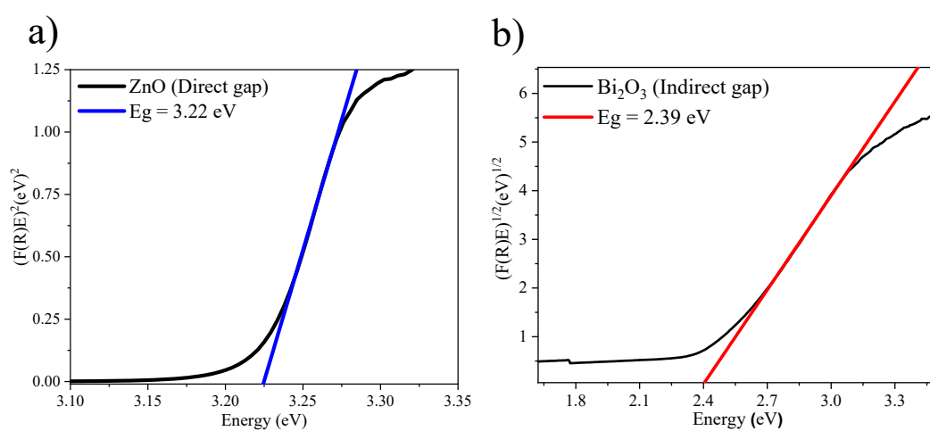
Fig. S1 Determination of the energy band gap of a) ZnO and b) Bi 2 O 3 films.
