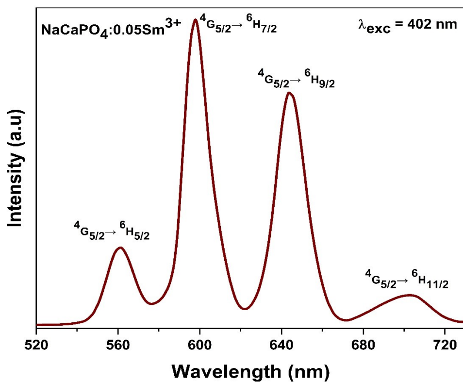
Fig. A1: The PL characteristics behaviour of NaCaPO 4 :0.05Sm 3+ at 402 nm excitation wavelength.
