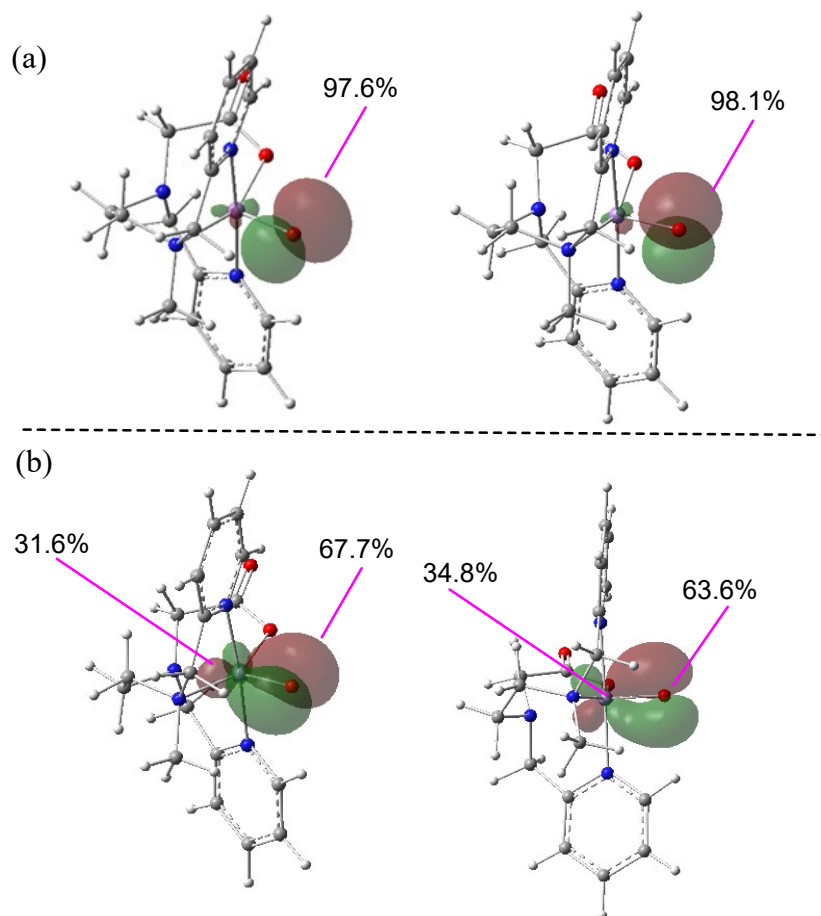
Fig. S1 Spatial plots of two lone pair orbitals with p character for (a) \alpha -spin and (b) \beta -spin electrons on the oxygen ligand in [\text{Mn}^{\text{IV}}(^{18}\text{O})(\text{mcbpen})]^+ (complex 3 ), as determined by NLMO calculations.
