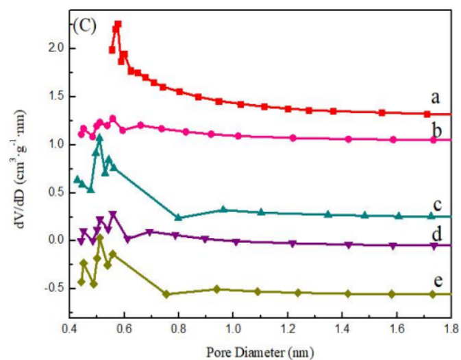
Fig.1s pore size distribution curve (microporous)
