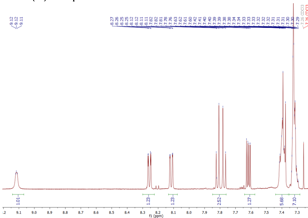
Figure S6. 1 H NMR spectrum of L (CDCl 3 ), selected range.
