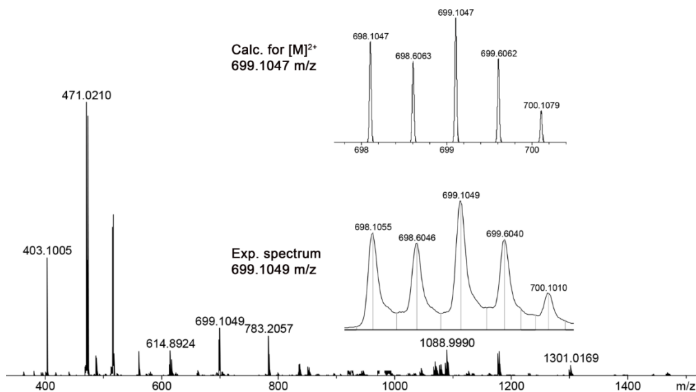
Figure S21. Experimental and calculated ESI + mass spectra of 5.
