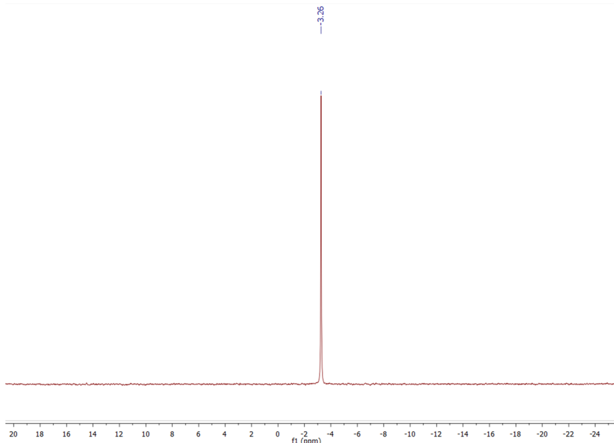
Figure S12. ^{31}\text{P}\{^1\text{H}\} NMR spectrum of L ( \text{CDCl}_3 ), selected range.
