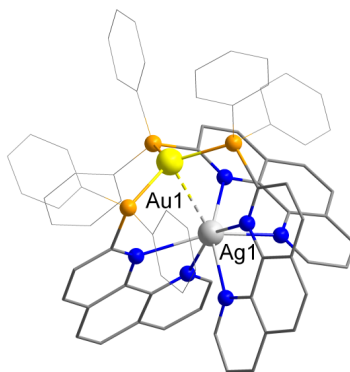
Figure S5. Molecular structure of 5 ·0.5Et 2 O determined by sc-XRD analysis (the H atoms, PF 6 - counterions and solvent molecules are omitted). Selected bond lengths (Å) and angles (°): Au1···Ag1 2.9294(12), Au1–P1 2.3575(18), Au1–P2 2.3575(19), Au1–P3 2.3576(18); P2–Au1···Ag1 88.82(5), P3–Au1···Ag1 88.82(5), P1–Au1···Ag1 88.82(5), P1–Au1–P3 119.957(4); P2–Au1–P3 9.956(4).
