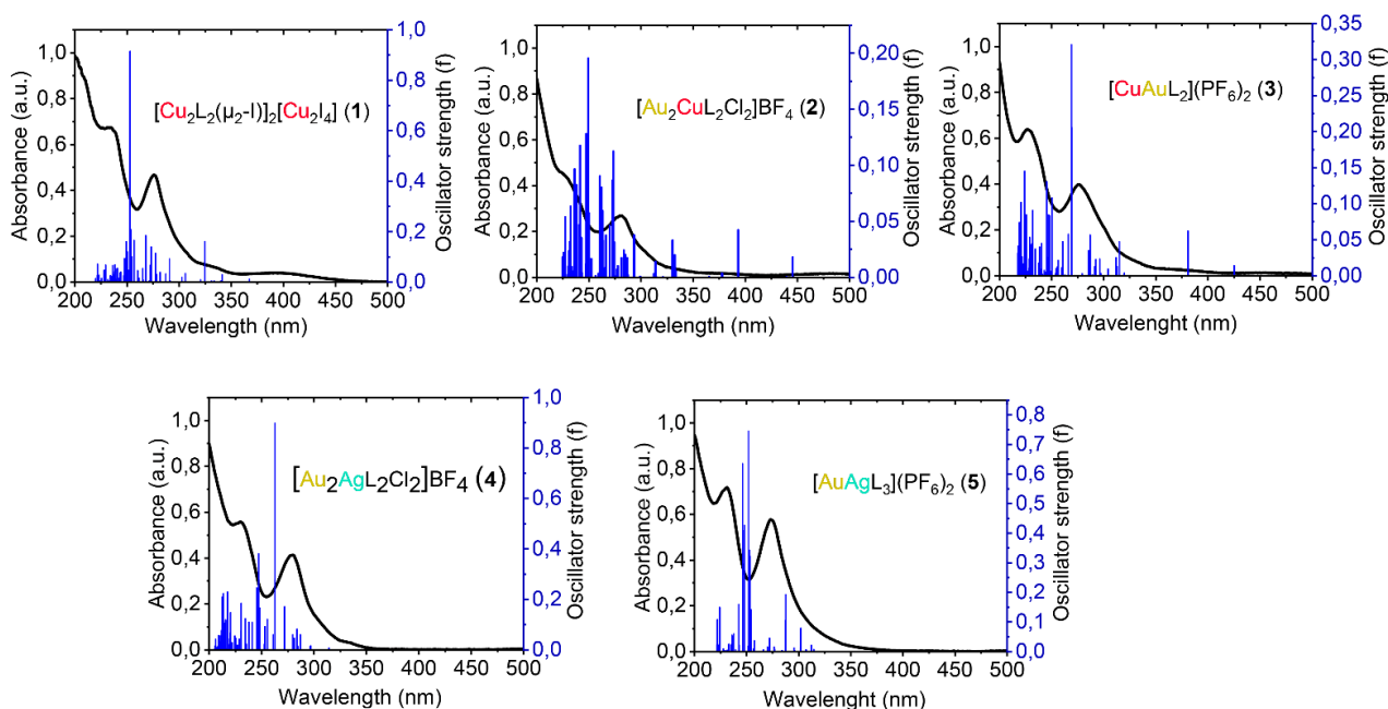
Figure S33. Experimental electronic absorption spectra (solid black curves) of 1–5 (MeCN, 298 K) and electronic transitions (vertical blue bars) calculated for the [\text{Cu}_2\text{L}_2(\mu_2\text{-I})]^{2+} , [\text{Au}_2\text{CuL}_2\text{Cl}_2]^+ , [\text{CuAuL}_2]^{2+} , [\text{Au}_2\text{AgL}_2\text{Cl}_2]^+ and [\text{AuAgL}_3]^{2+} cations, respectively 5 calculated at CAM-B3LYP/def2-TZVP//B3LYP-D4/ZORA-def2-TZVP level.
