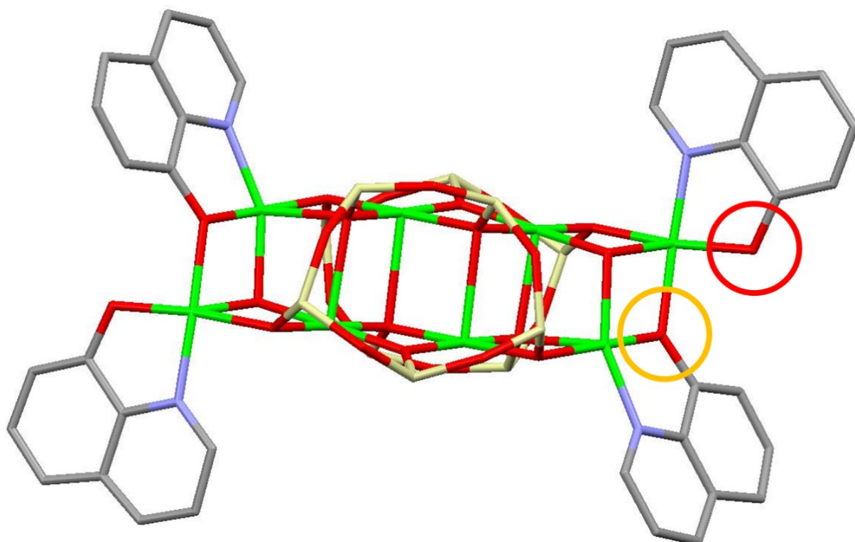
Figure S10. Top view of complex 2. Phenyl groups at silicon atoms and hydrogen atoms are omitted for clarity. Circles are to represent bridging (orange circle) and chelating (red circle) ligation styles of 8-hydroxyquinolate fragments.
