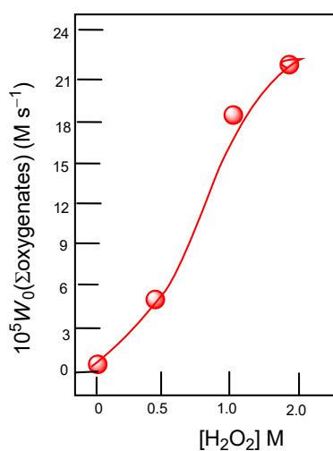
Figure S16. Dependence of the initial rate of oxygenate (sum cyclohexanol+cyclohexanone) formation W_0 in the oxidation of cyclohexane (0.46M) with hydrogen peroxide catalyzed by compound 1 ( 5 \times 10^{-4} M) in MeCN up to 2.5ml on concentration of hydrogen peroxide
