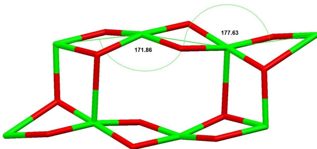
Figure S11. Metal oxide fragment in complex 2.
