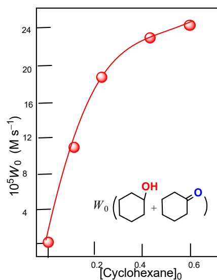
Figure S13. Dependence of the initial rate of oxygenates formation W_0 on initial concentration of cyclohexane in oxidation of cyclohexane with hydrogen peroxide (2.0 M, 50 % aqueous, 0.32ml) catalyzed by compound 1 ( 5 \times 10^{-4} M, 3mg) in MeCN (up to 2.5ml) at 50 °C. Concentrations of cyclohexanone and cyclohexanol were determined after reduction of the aliquots with solid PPh 3 .
