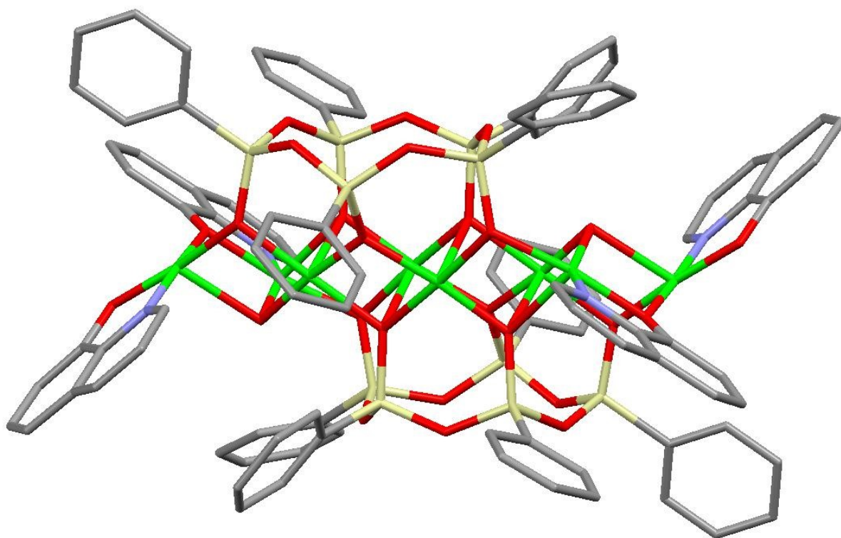
Figure S9. Side view of complex 2. Hydrogen atoms are omitted for clarity.
