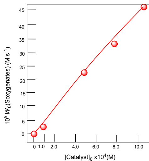
Figure S14. Dependence of the initial rate of oxygenate (sum cyclohexanol+cyclohexanone) formation W_0 in the oxidation of cyclohexane (0.46M) with hydrogen peroxide (2.0 M, 50 % aqueous) catalyzed by compound 1 in MeCN up to 2.5ml, at 50° C on the initial concentration of catalyst
