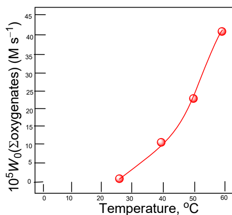
Figure S15. Dependence of the initial rate of oxygenate (sum cyclohexanol+cyclohexanone) formation W_0 in the oxidation of cyclohexane (0.46M) with hydrogen peroxide (2.0 M, 50 % aqueous) catalyzed by compound 1 ( 5 \times 10^{-4} M) in MeCN up to 2.5ml on reaction temperature
