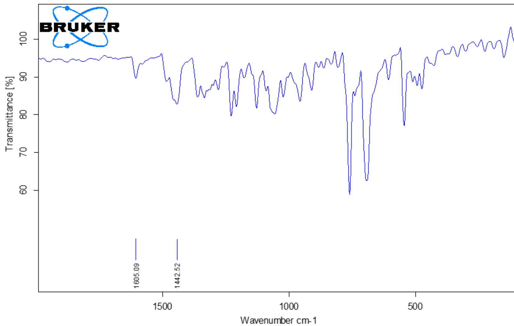
Figure S9. IR spectrum of ligand (L)
